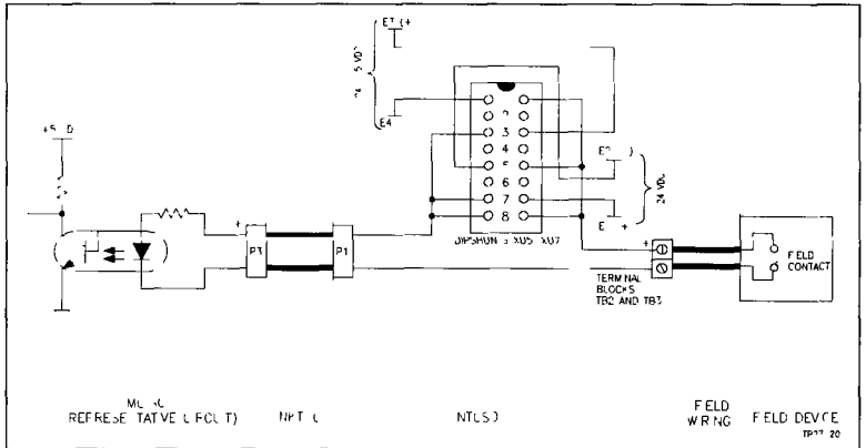
Figure A 1 NTCS02 Dipshunt for Digital Inputs
