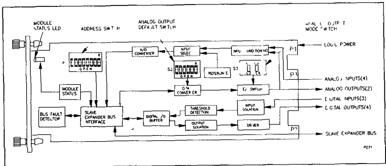
Figure 2.1 Control I/O Slave Module Block Diagram
