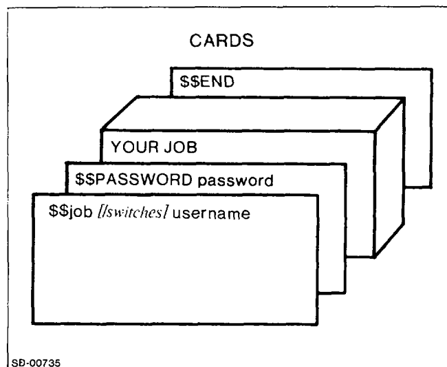
Figure D-1. Stacked Format for Batch Jobs
