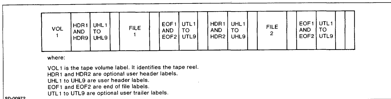
Figure 2-9. Labeled Magnetic Tape
