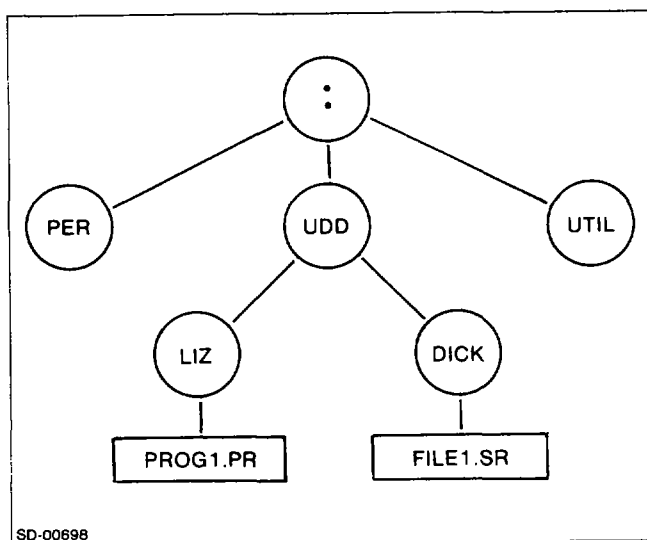
Figure 2-7. Search List Example
