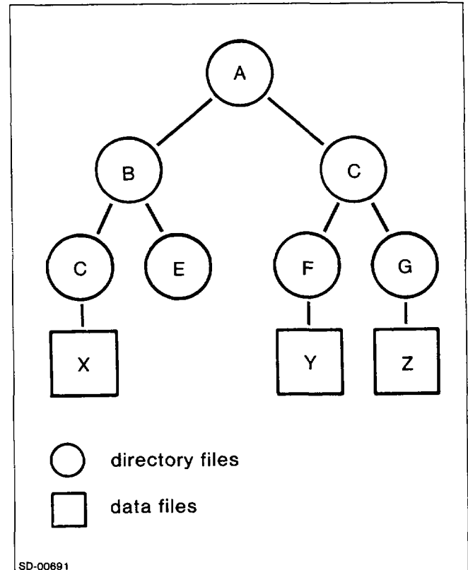
Figure 2-5. A Directory Subtree
