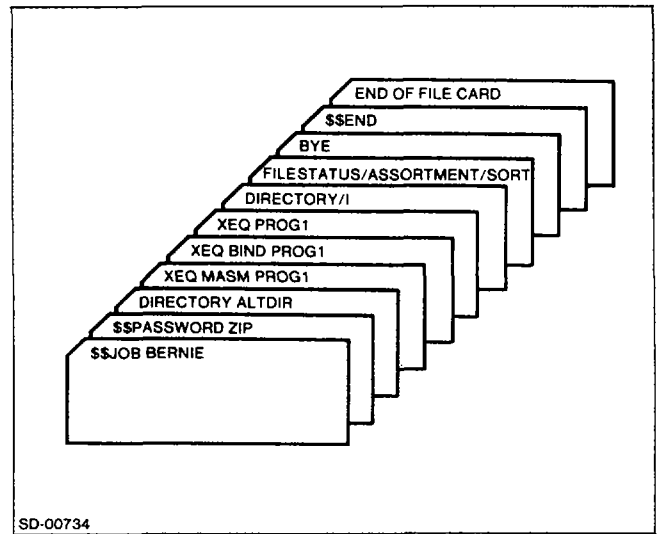
Figure D-2. Sample Batch Job in Stacked Format
