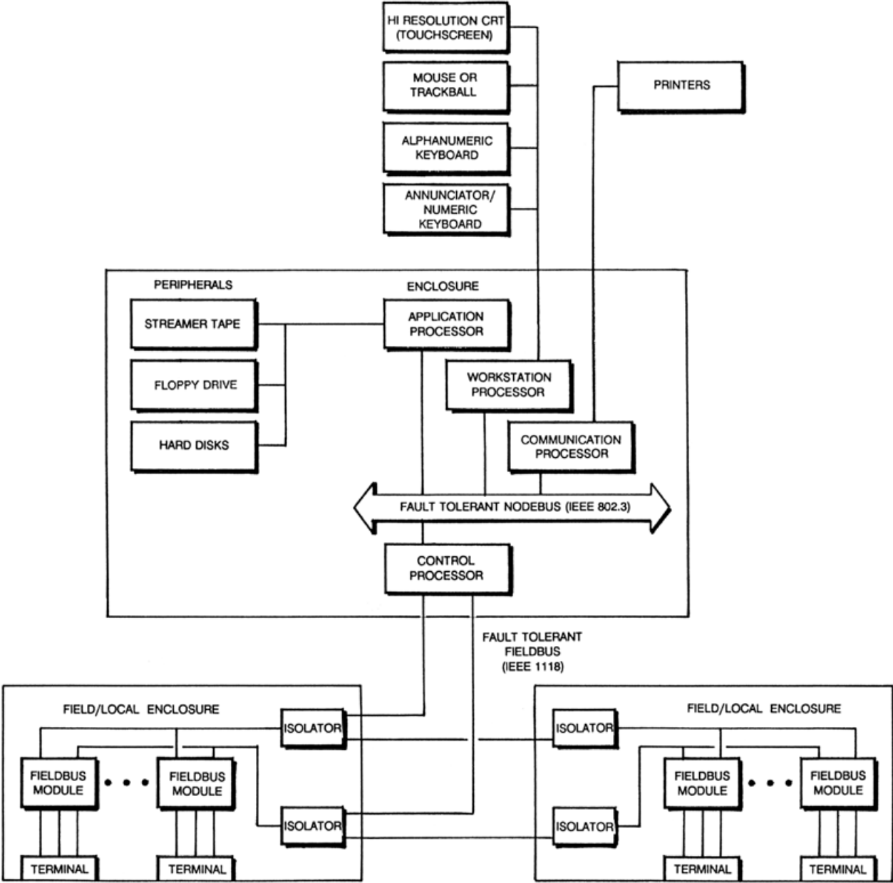
Figure 4. Typical I/A Series Single Node System
