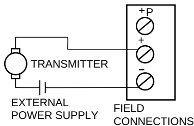
EXTERNAL POWERED TRANSMITTER
