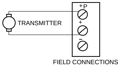
MODULE POWERED TRANSMITTER
