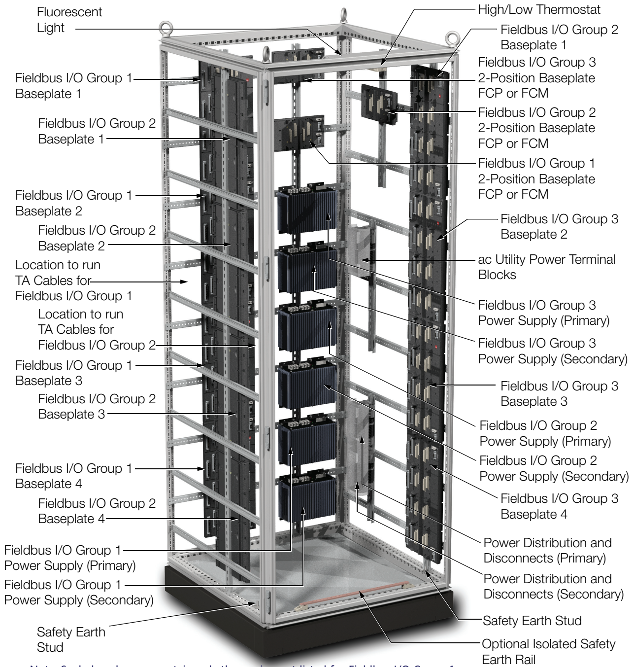
Figure 1. G15 System Enclosure, Front Left View
