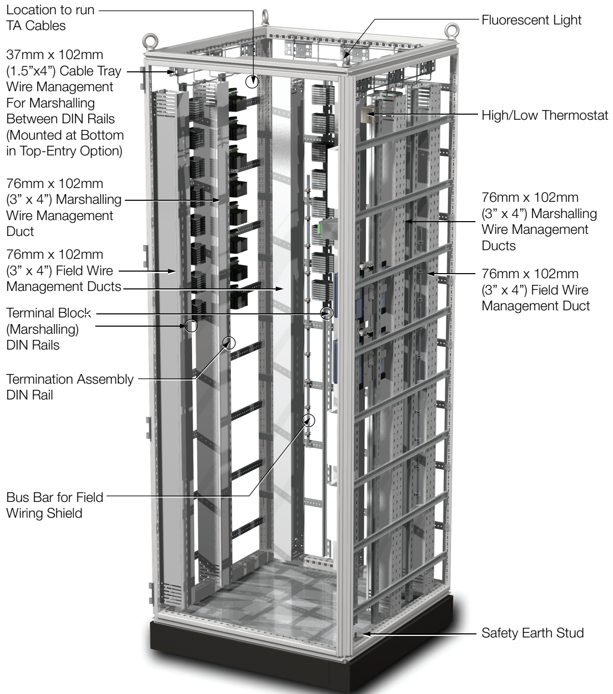
Figure 3. G16 Termination Enclosure with Marshalling Option, Front Right View, Bottom Entry
