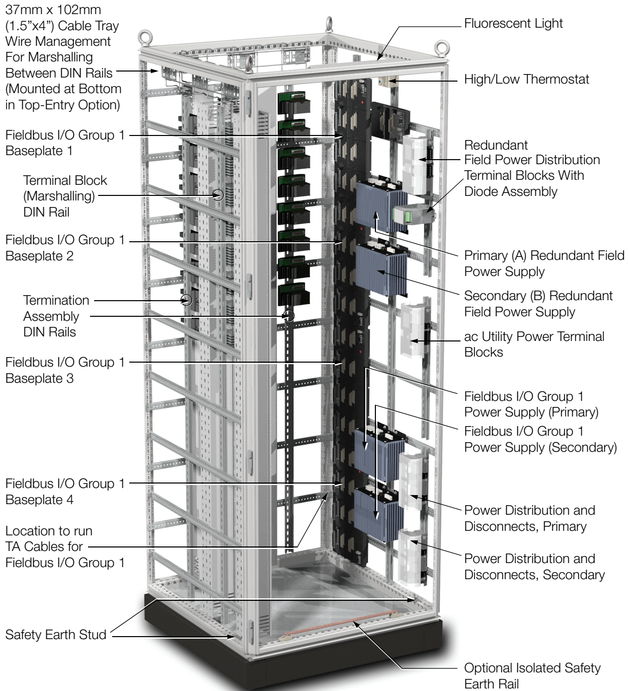
Figure 1. G17 System and Termination Enclosure, Front Left View
