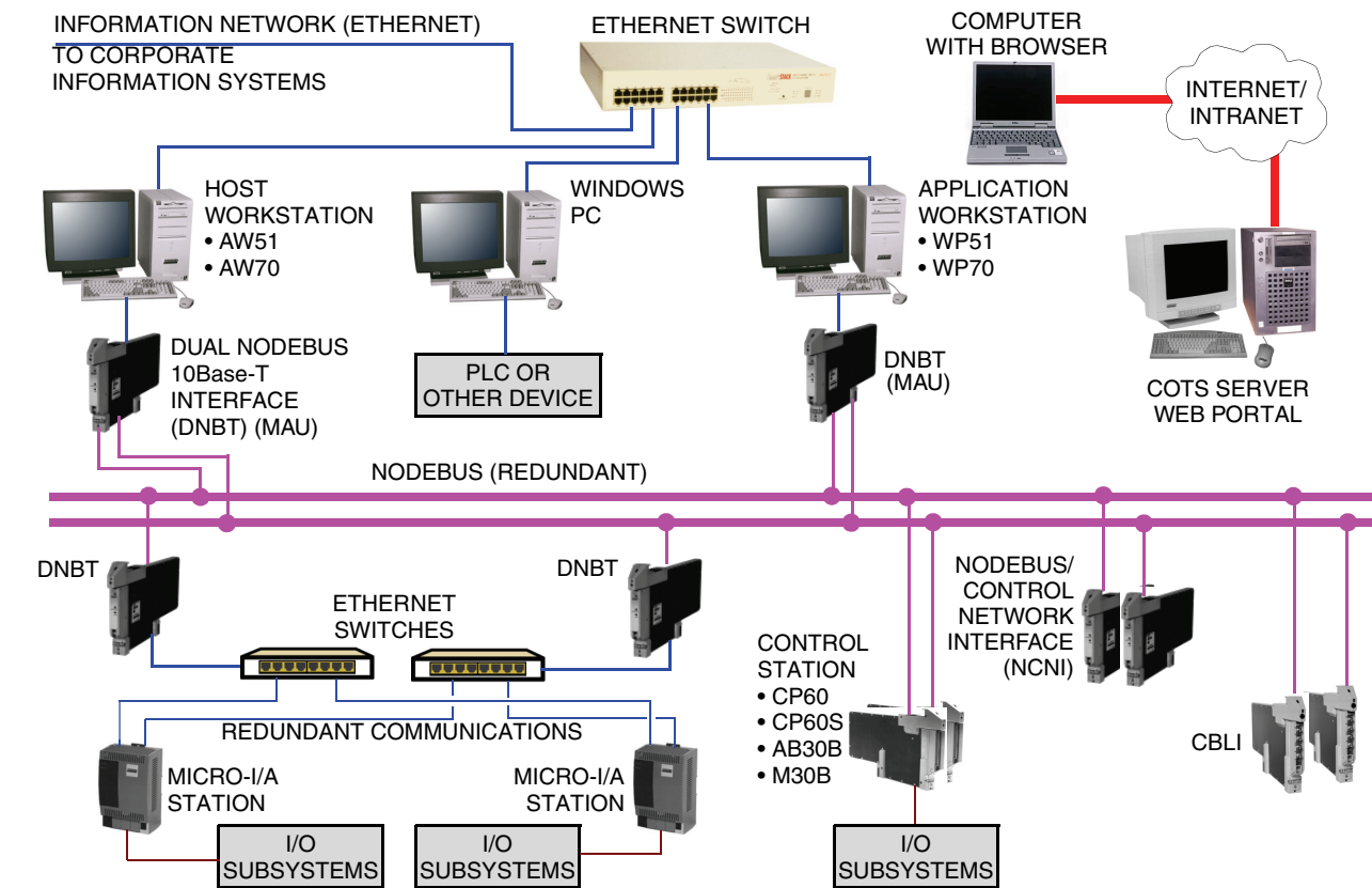
Figure 5. Details of I/A Series Redundant Nodebus Control - Example Diagram
