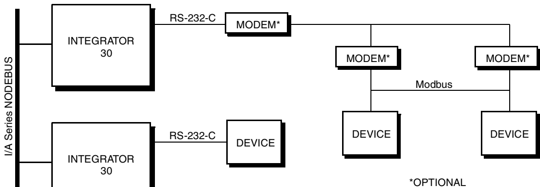
Figure 1. Typical Integrator 30 Configurations
