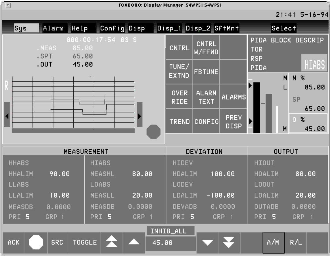
Figure 15. Example of Block Detail Display for PIDA Block
