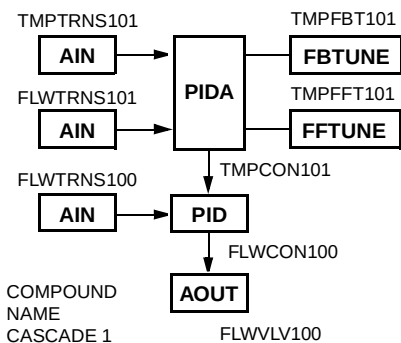
Figure 6. Example of a Compound Control Scheme
