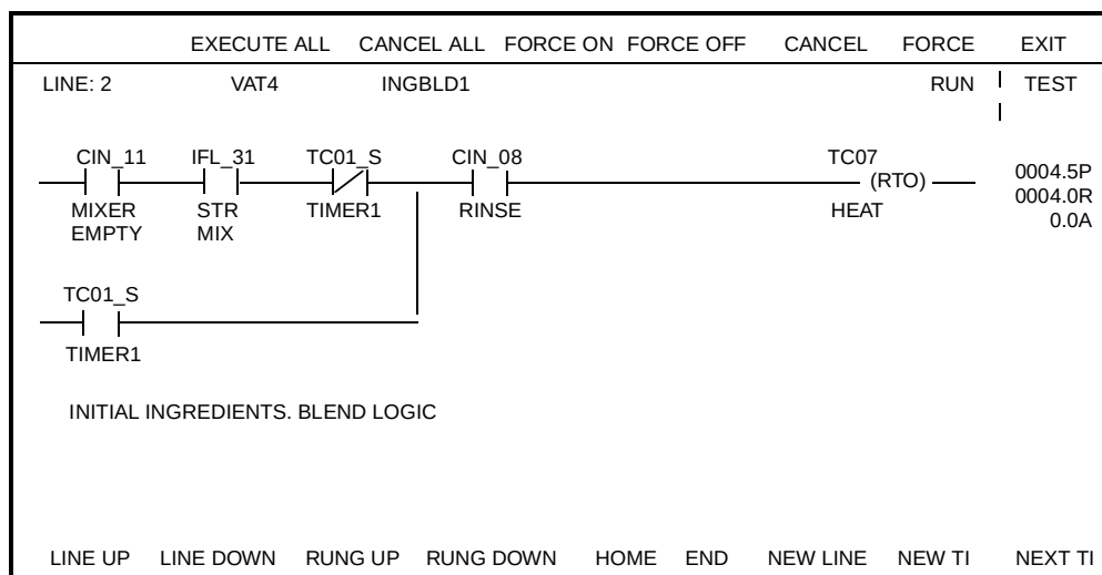
Figure 9. Sample Ladder Diagram in PLB Monitor for Testing
