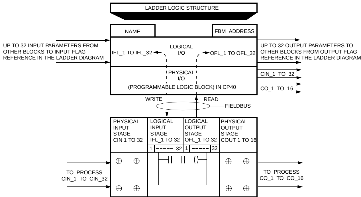
Figure 7. Programmable Logic Block
