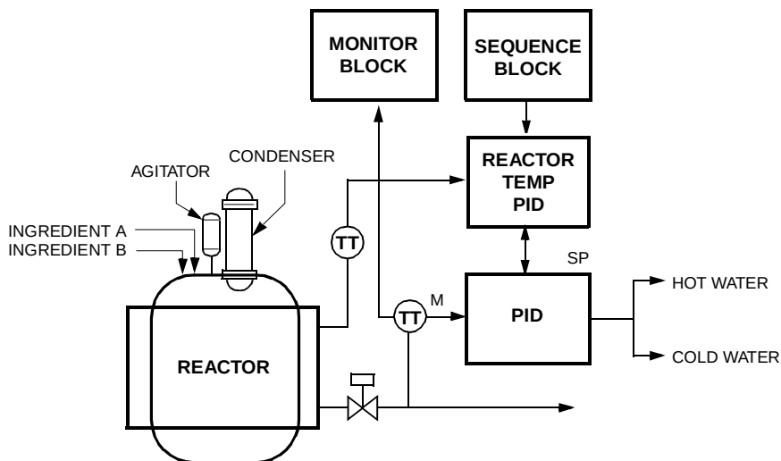
Figure 11. Sample Control Loops
