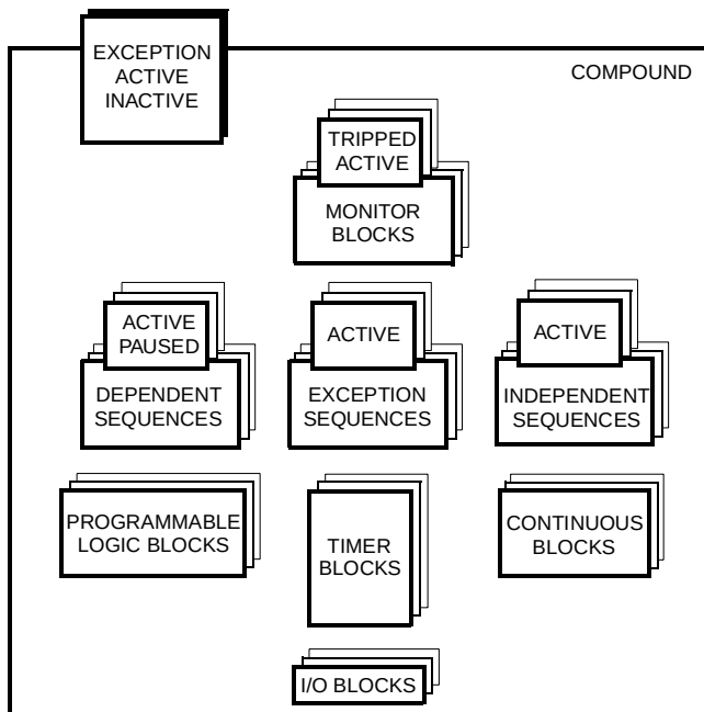
Figure 10. Example of Compound Contents
