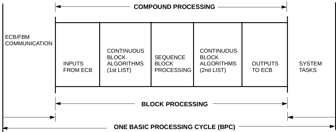
Figure 4. Basic Block Processing (BPC)
