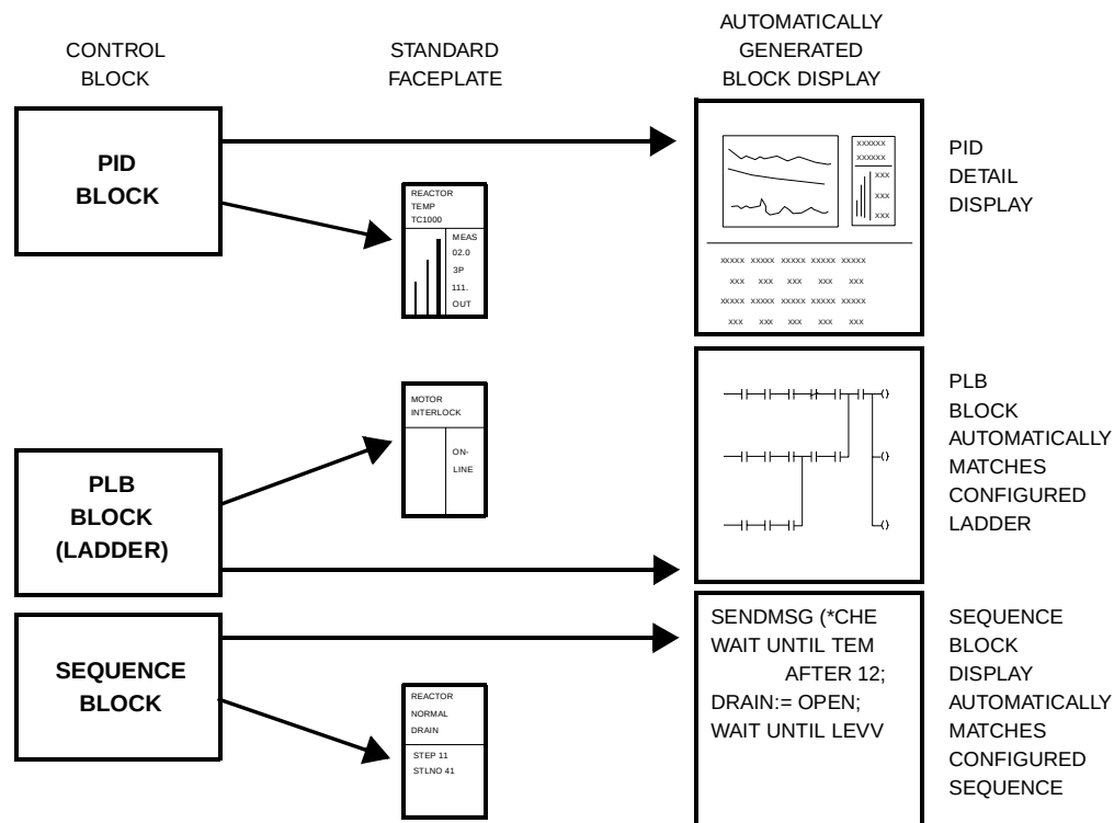
Figure 14. Automatically Generated (Default) Block Detail Displays
