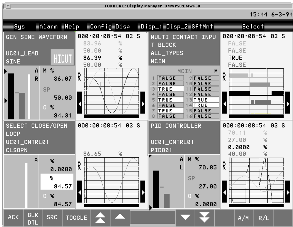
Figure 16. Typical Group of Faceplates and Trends
