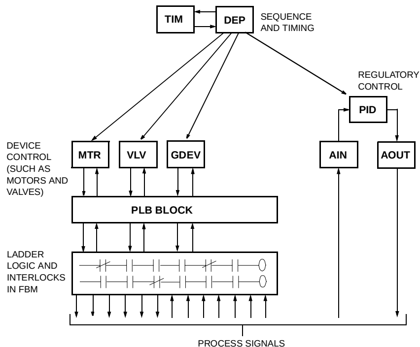
Figure 3. Total Integration in a Single Control Station
