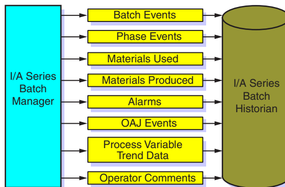
Figure 5. Batch History (EBR)
