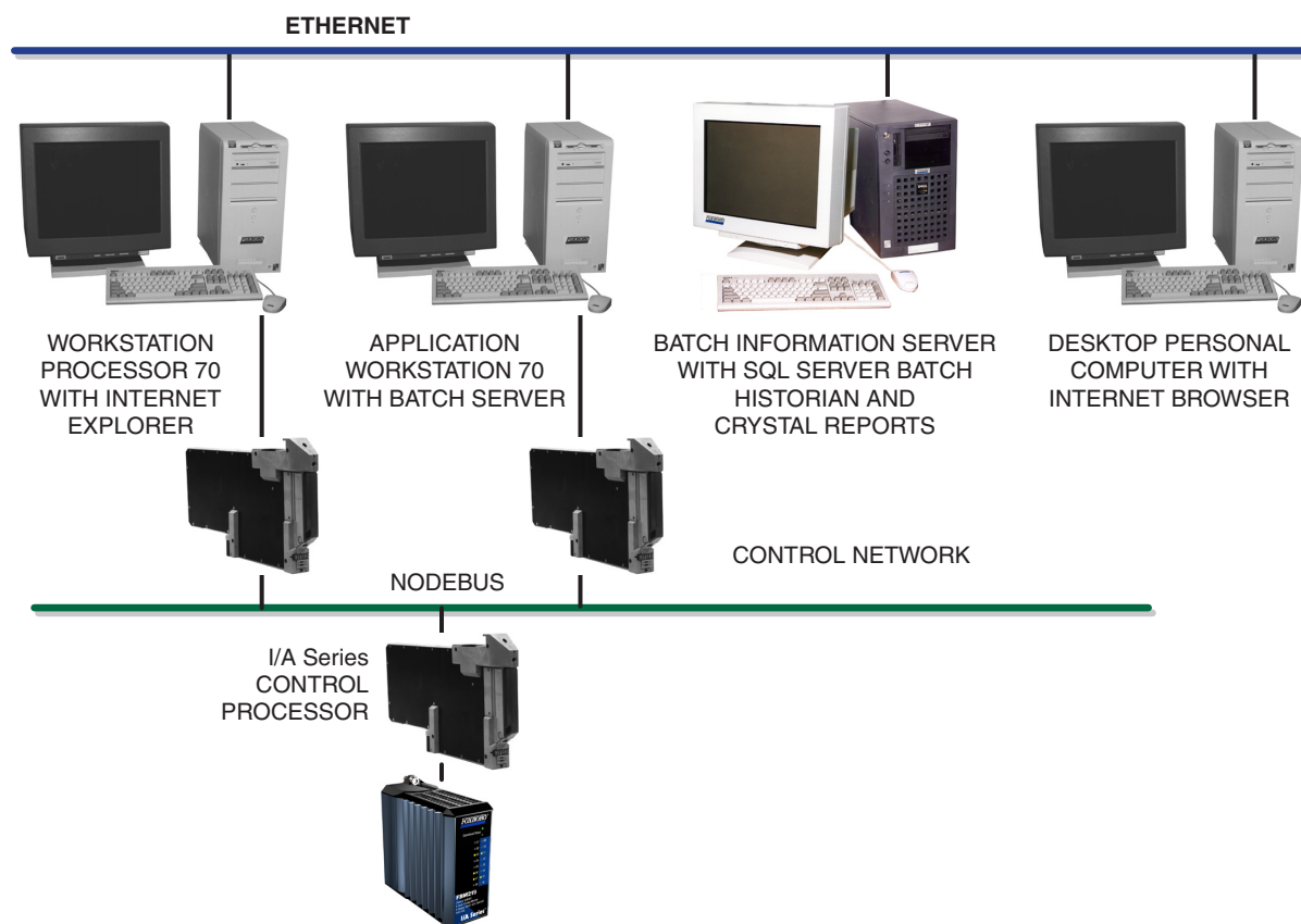
Figure 13. Windows NT Batch Reporting System Configuration
