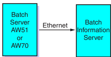
Figure 4. Batch System Architecture
