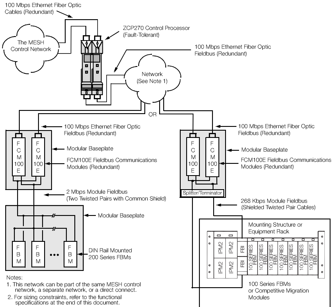
Figure 2. Typical FCM100E Network Configuration (Simplified)
