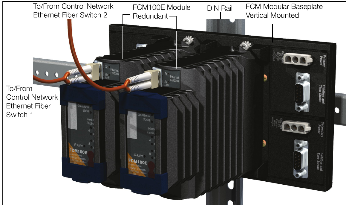
Figure 1. Redundant FCM100E Module on DIN Rail Mounted Modular Baseplate
