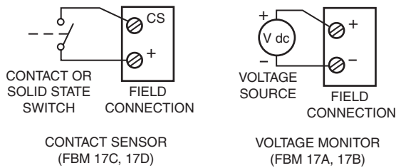
Figure 3. Digital Input Configurations
