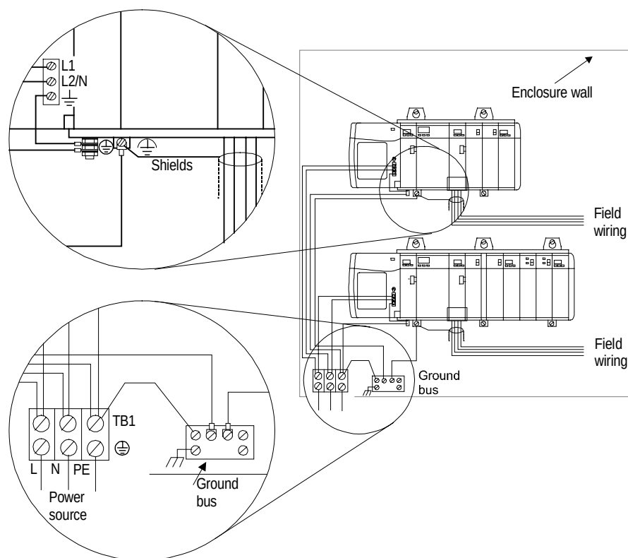
Grounding Configuration
