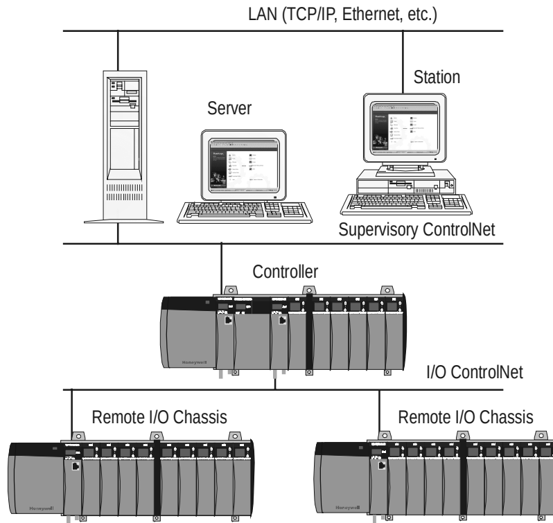
ControlNet topology
