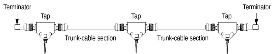
ControlNet trunk sections
