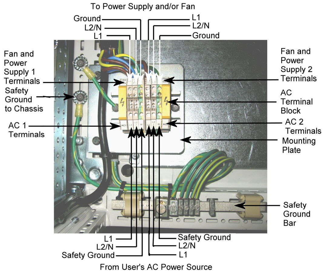
Figure 8 Typical power and ground connections to AC terminal block in Series C cabinet
