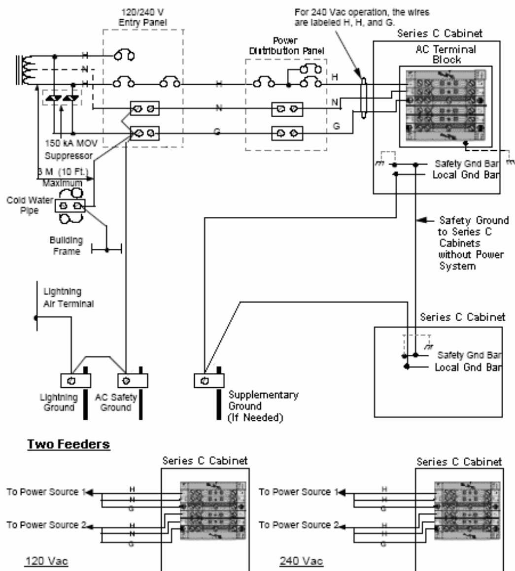
Figure 11 Typical power and ground connections for Series C cabinet.
