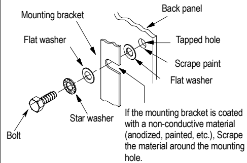
Alternative bolt mounting of chassis to the back panel
