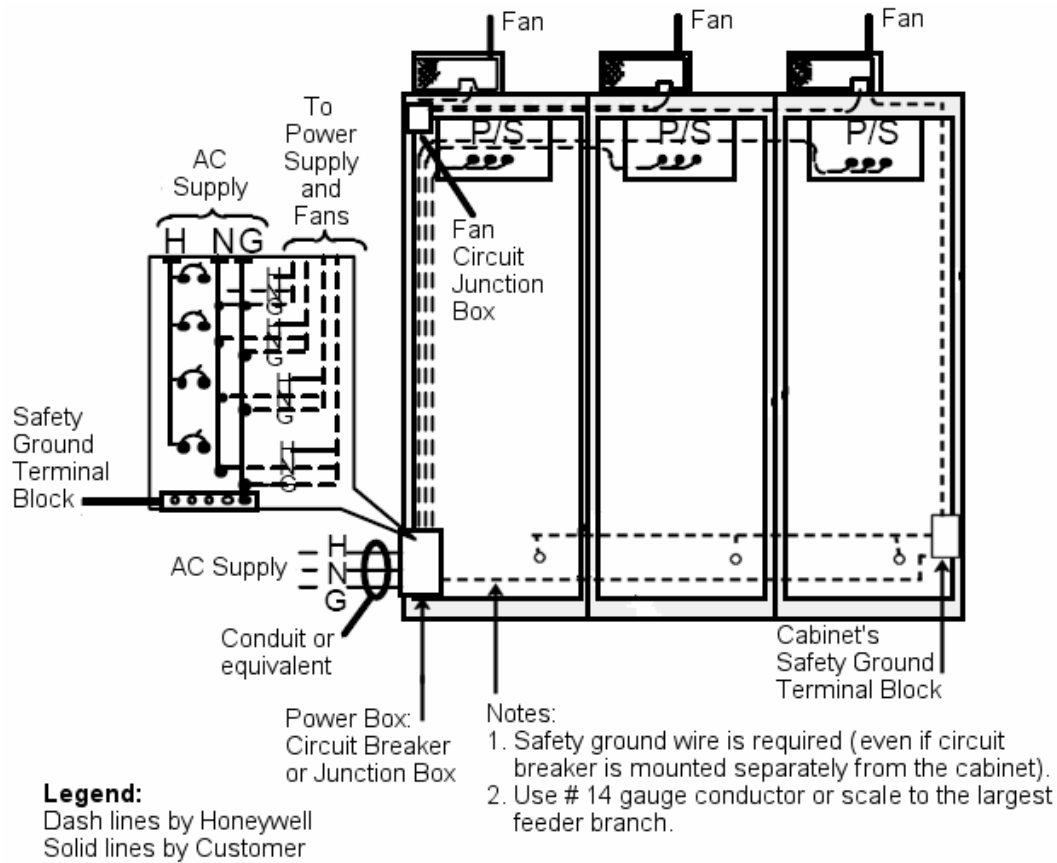
Figure 14 Typical PM cabinet safety ground connections.
