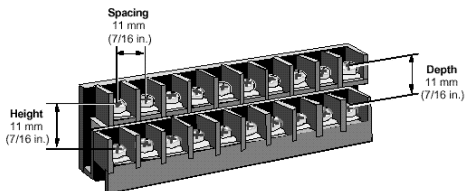
Fixed-Screw Terminal Connector for Standard Type FTA
