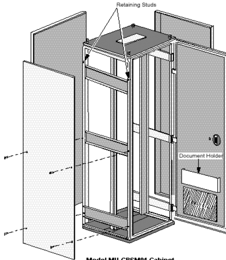
Model MU-CBSM01 Cabinet
