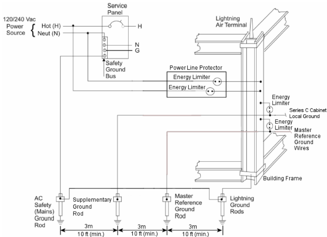
Figure 6 Typical AC power source through mains panel with safety ground bus, AC safety (mains) ground, supplementary ground, master reference ground, and lightning ground rods.
