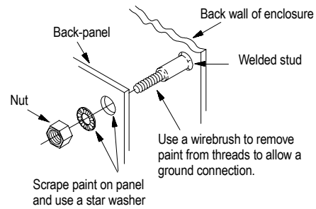
Stud mounting of the back panel to the enclosure back wall.
