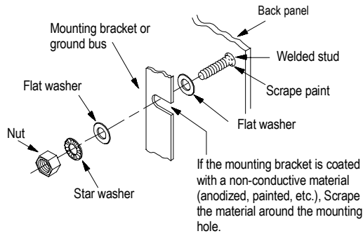
Stud mounting of a ground bus or chassis to the back panel
