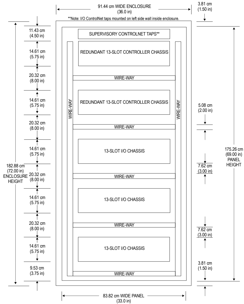
Large-scale system enclosure configuration example, 1-of-2
