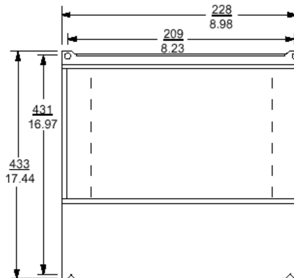
7-Slot Card File Mounting Dimensions
