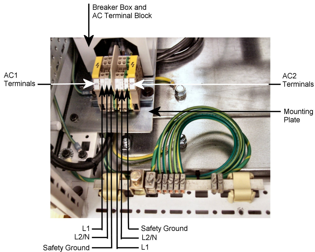
Figure 9 Typical power and ground connections to optional breaker box and AC terminal block in Series C cabinet
