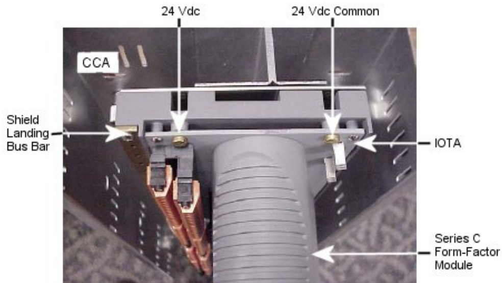
Figure 1 Top View of Carrier Channel Assembly with IOTA and resident Series C form-factor module installed
