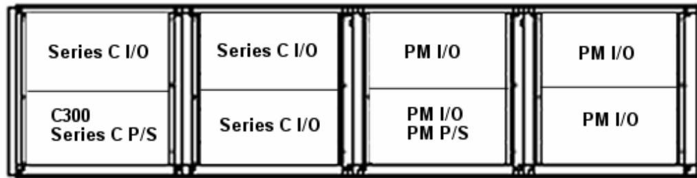
Figure 12 Quad dual access cabinet complex example with C300, Series C power supply, Series C I/O, PM power supply, and PM I/O in Series C and PM cabinets, respectively
