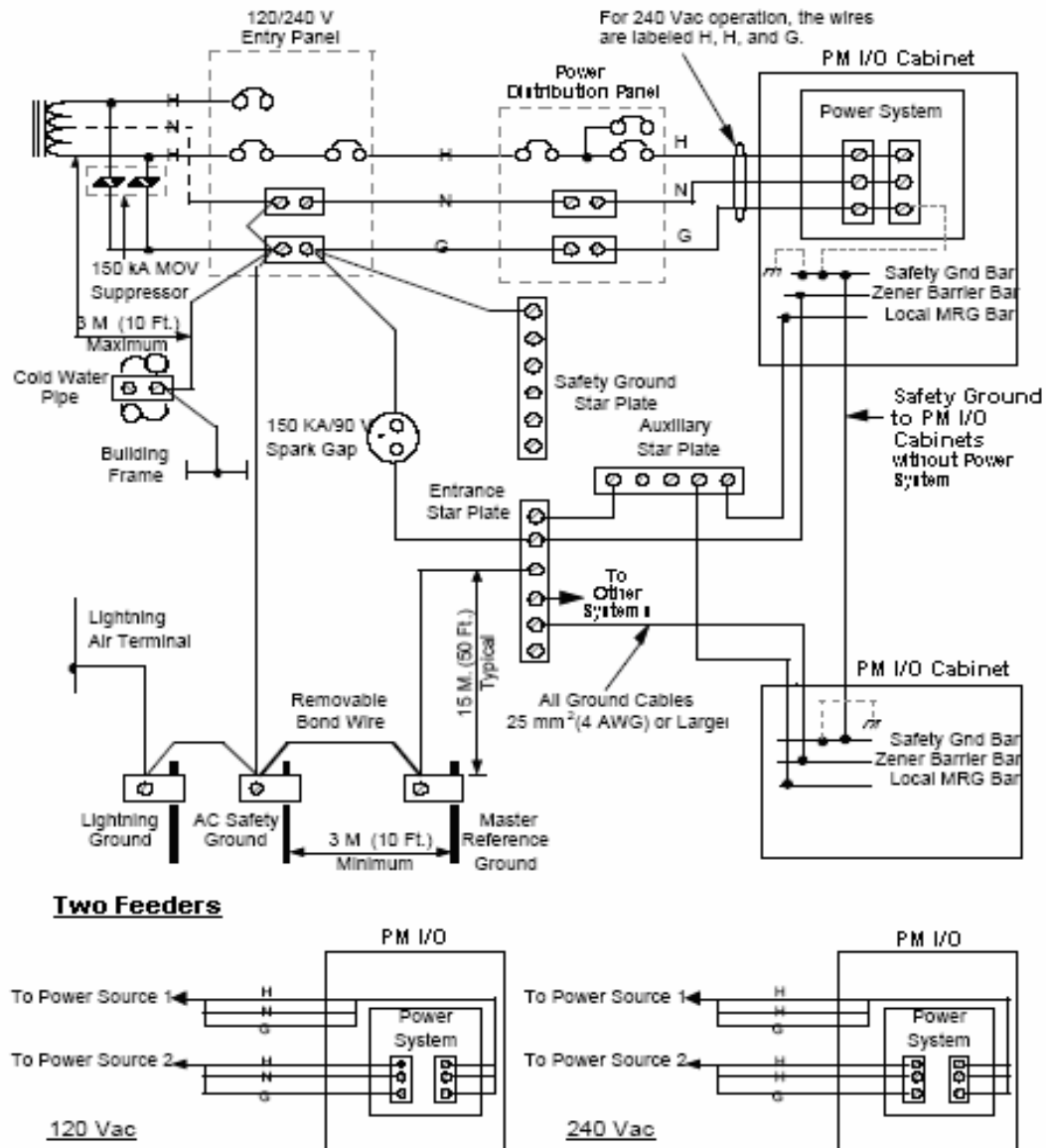
Figure 13 Typical power and ground connections for PM I/O cabinet that is non-EC compliant.
