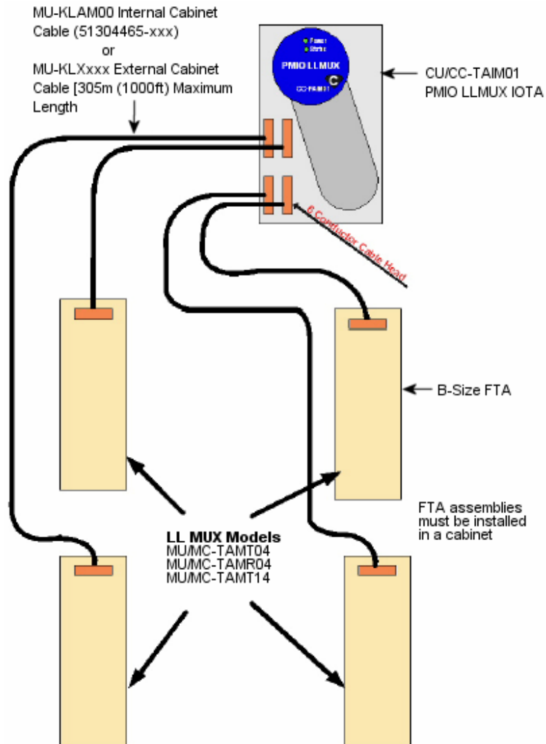
Figure 3 LLMUX FTA used with Series C LLMUX IOTA
