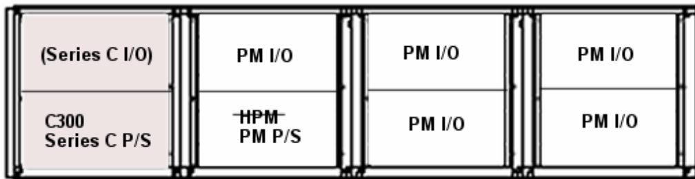
Figure 16 Quad dual access cabinet complex example with C300 and Series C power supply in Series C cabinets replacing HPM in PM cabinets with PM power supply and PM I/O
