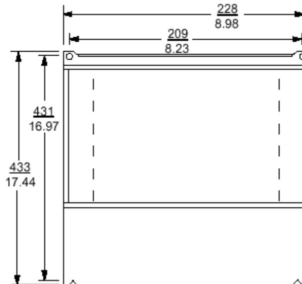
7-Slot Card File Mounting Dimensions
