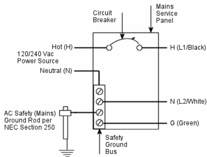
Figure 5 Typical AC power source through mains panel with safety ground bus and AC safety (mains) ground rod.
