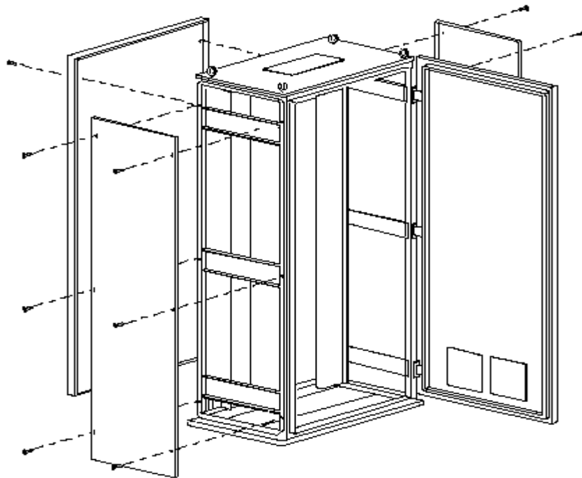
Model MU-C8SFR1 Cabinet
