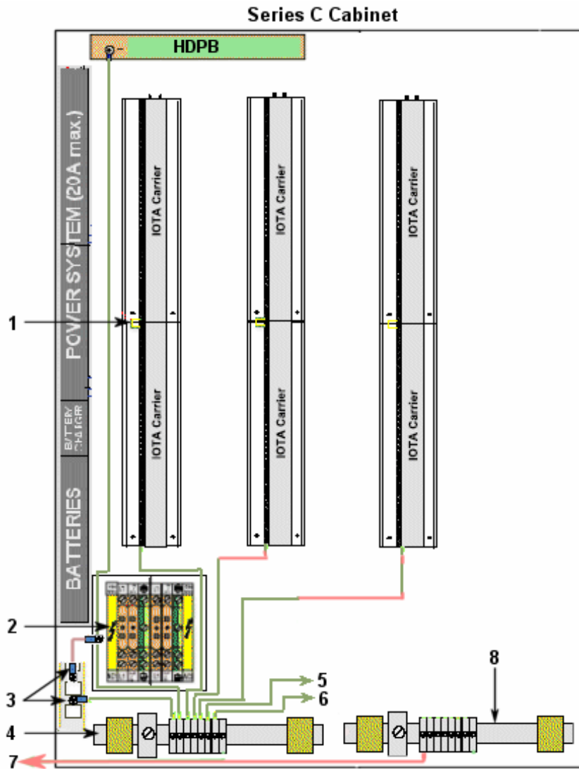
Figure 7 Typical safety ground connections in Series C cabinet
