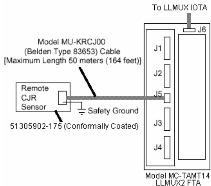
Figure 4 Remote CJR sensor connected to LLMUX2 FTA MC-TAMT14
