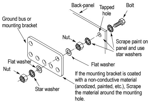
Bolt mounting of a ground bus or chassis to the back-panel.
