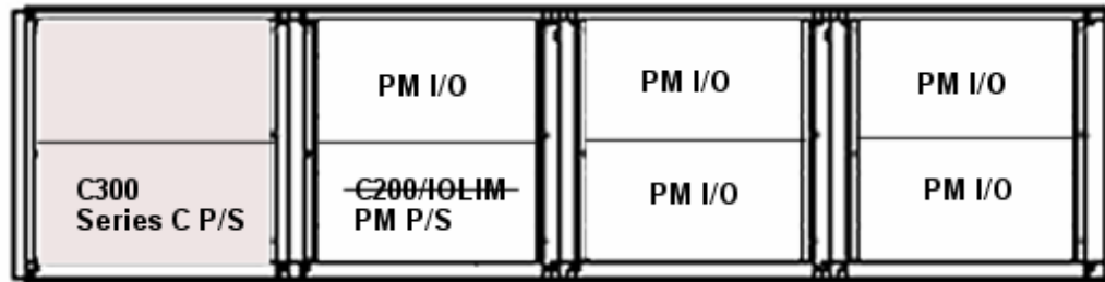
Figure 15 Quad dual access cabinet complex example with C300 and Series C power supply in Series C cabinets replacing C200/IOLIM in PM cabinets with PM power supply and PM I/O
