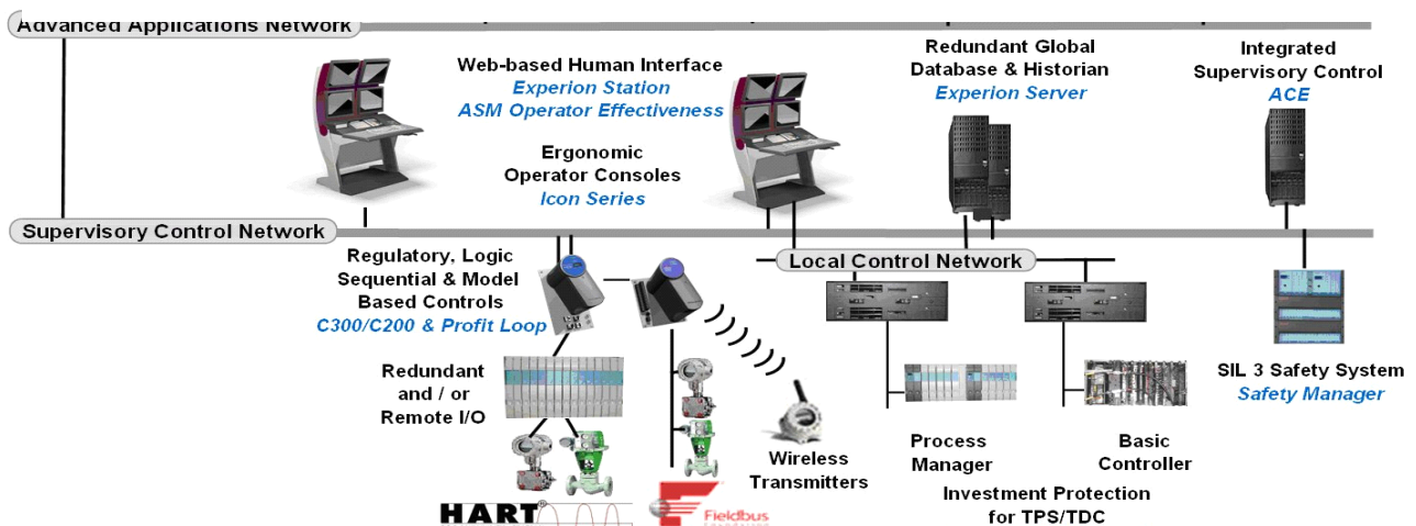
Figure 1. Sample Experion Architecture
