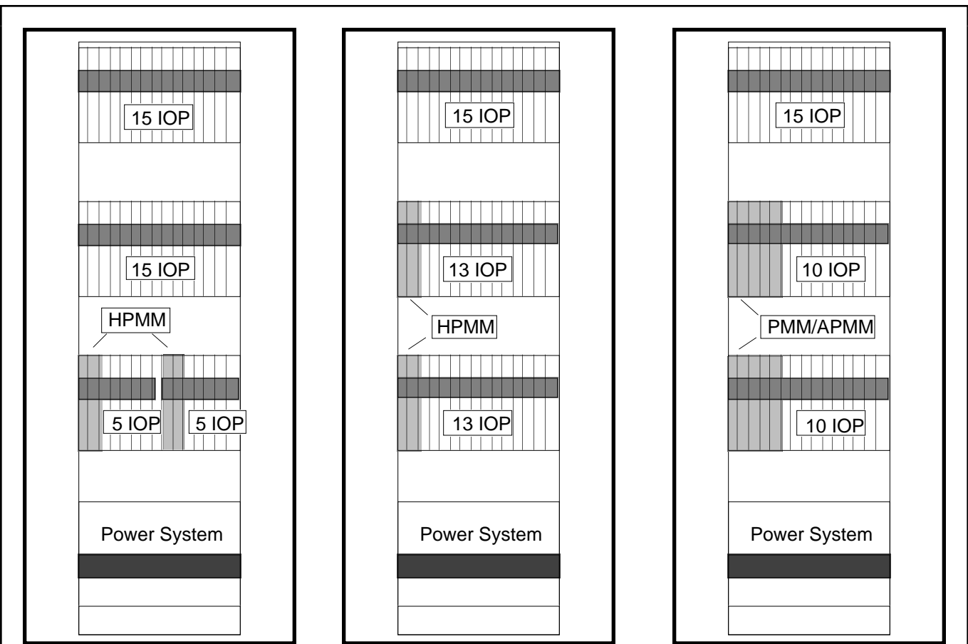
7-Slot HPM Cabinet
