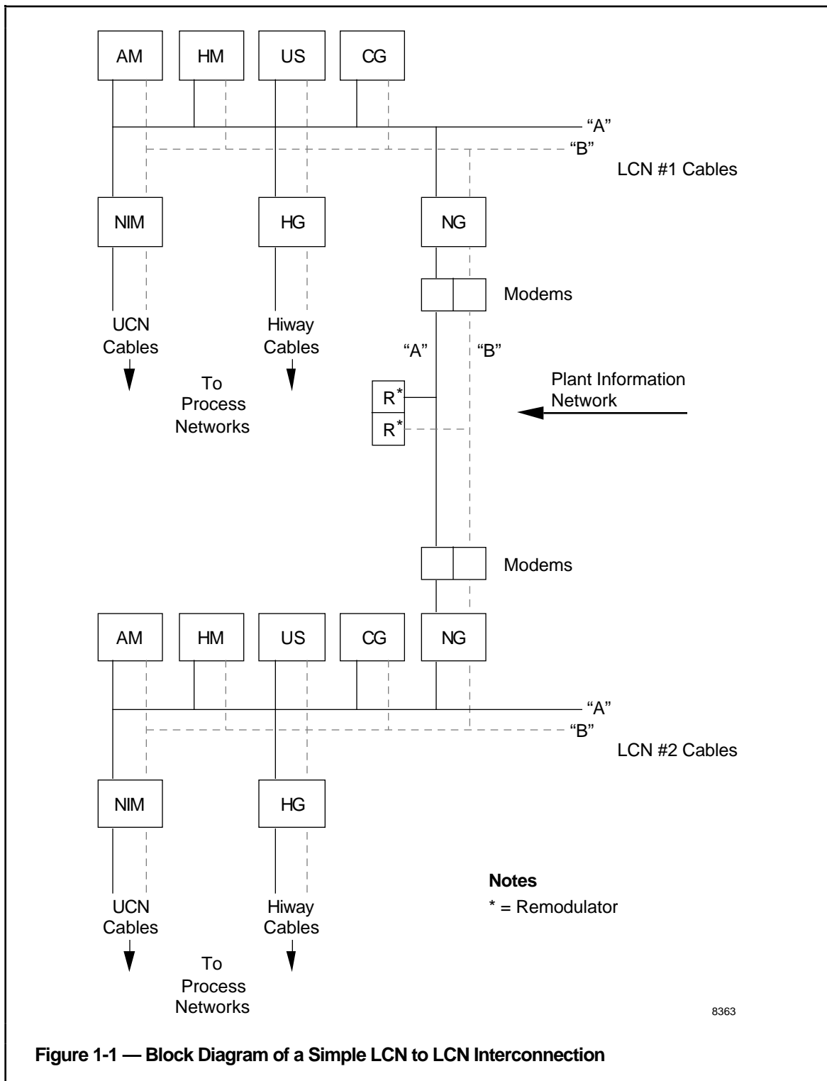
Figure 1-1 shows a simple interconnection between two LCN systems that uses both an "A" cable and a "B" cable for the PIN. The "B" cable is an option that improves system availability requirements in the event of "A" cable failure. Because this example uses a single NG at each LCN, the failure of either NG would cause the LCNs to lose communication.
