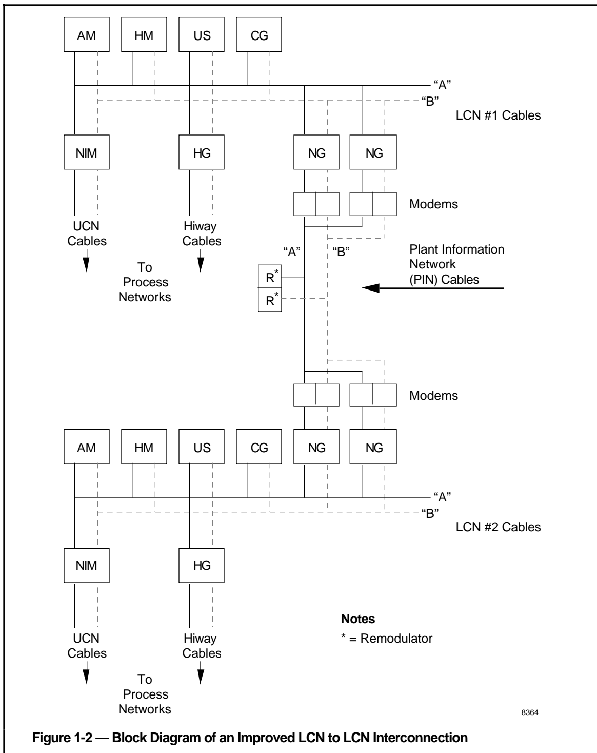
Figure 1-2 — Block Diagram of an Improved LCN to LCN Interconnection Figure 1-2 shows an improved interconnection that provides alternate routing capability by placing two NGs on each LCN. Note that the NGs are not redundant. Each NG is a separate node (on both the LCN and PIN networks) and software configuration determines what communication traffic runs on each and selects alternate paths for communication. This allows for continued system operation even if one NG should fail.
