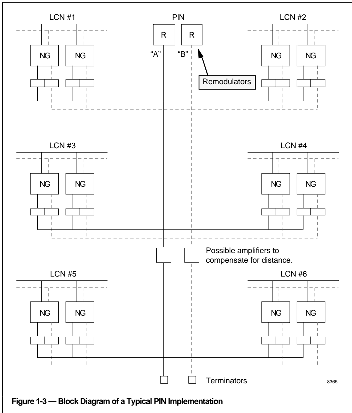
Figure 1-3 shows a broader application of the PIN. It illustrates how more than two LCNs could be interconnected. Note that this example still shows only two NGs on each LCN. The LCN software supports up to 10 NGs per LCN, thus permitting a wide variety of possible communications paths.
