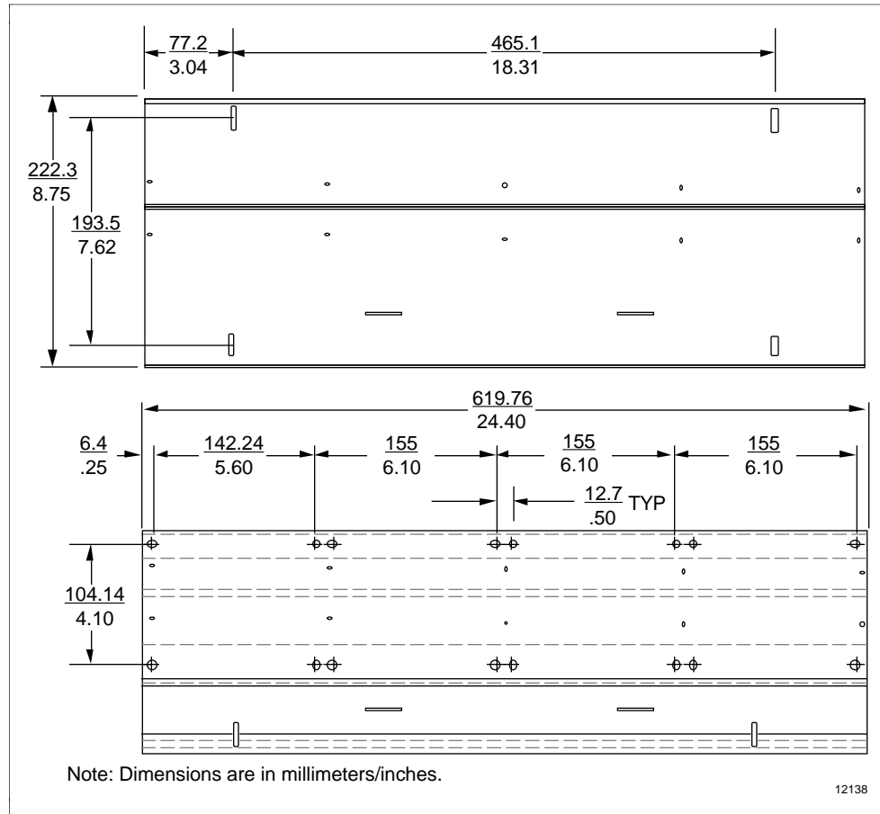
Figure 8-15 Horizontal FTA Mounting Channel Installation Holes
