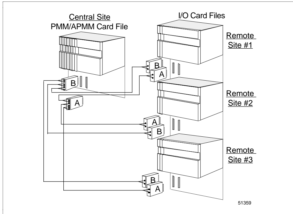
Figure 11-1 Standard I/O Link Extender Interconnections with Nonredundant PMM or APMM
