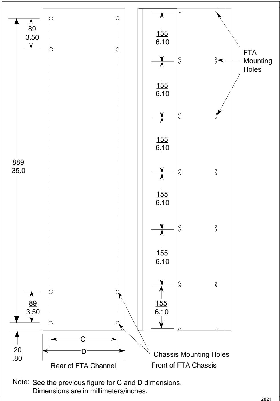
Figure 9-14 FTA Mounting Channel Mounting FTA Installation Holes
