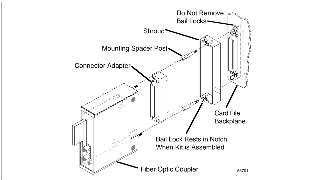
Figure 7-1 I/O Link Extender Adapter Kit
