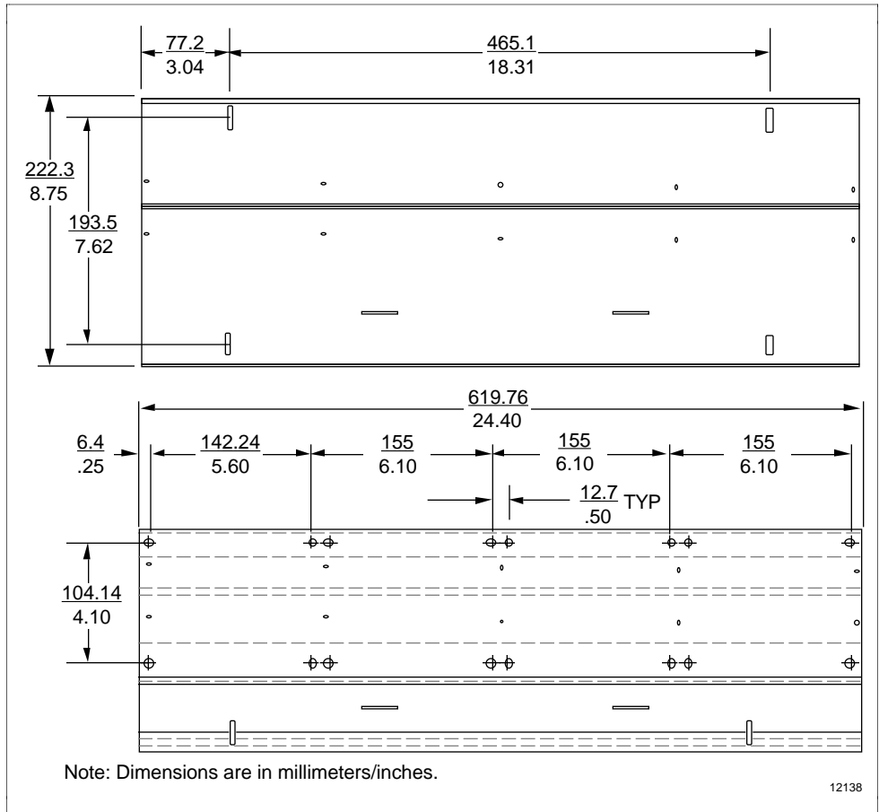
Figure 9-17 Horizontal FTA Mounting Channel Installation Holes
