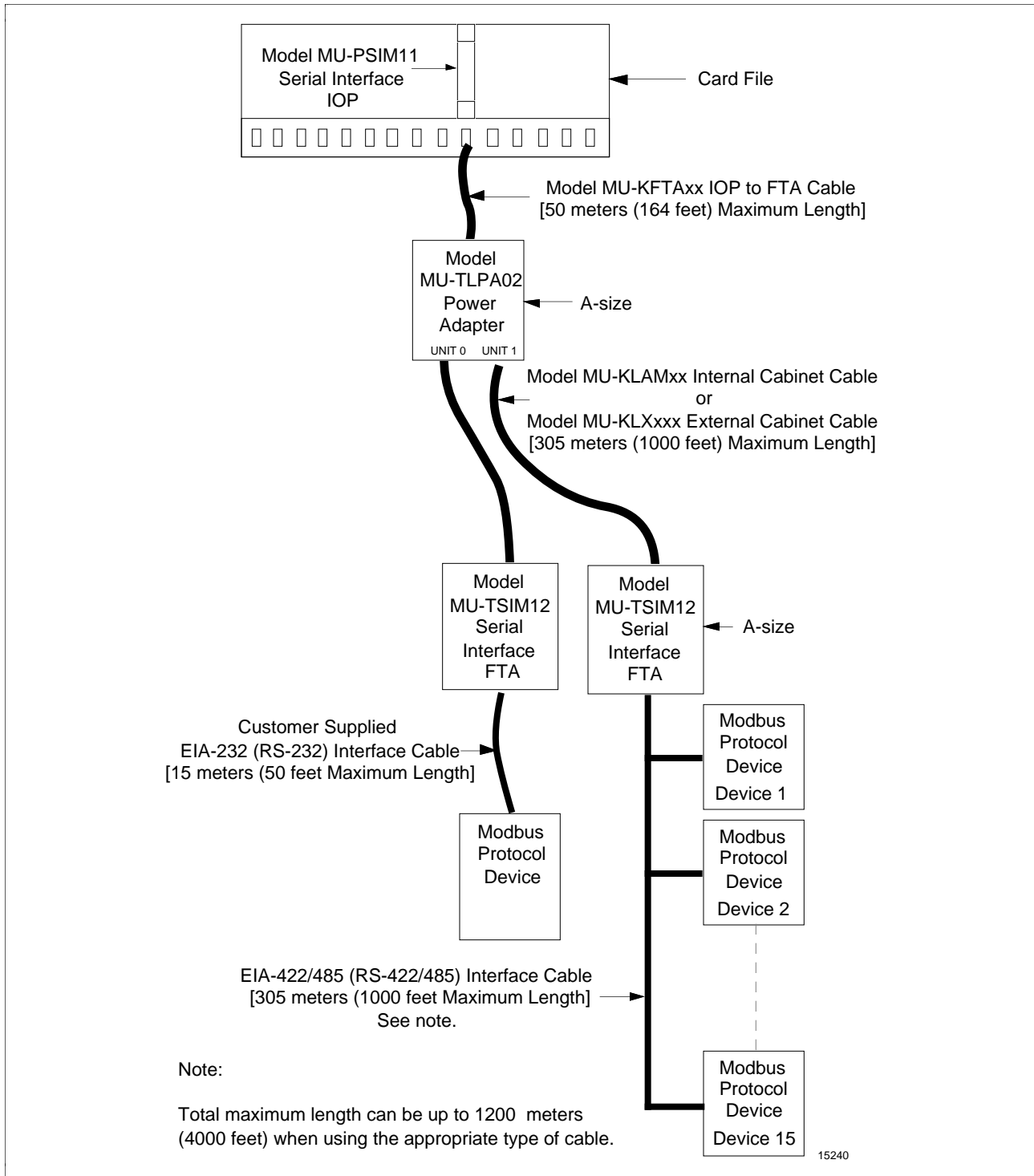
Figure 14-1 Model MU-TSIM12 Serial Interface FTA Interconnections—Non-CE Compliant
