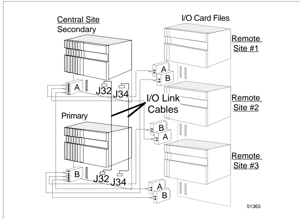
Figure 2-10 Standard I/O Link Extender Interconnections with Redundant PMMs or APMMs
