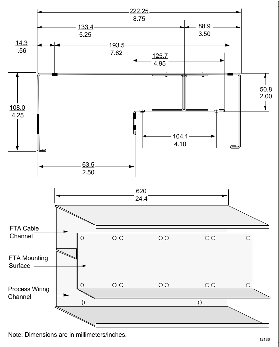
Figure 8-14 Horizontal FTA Mounting Channel Dimensions
