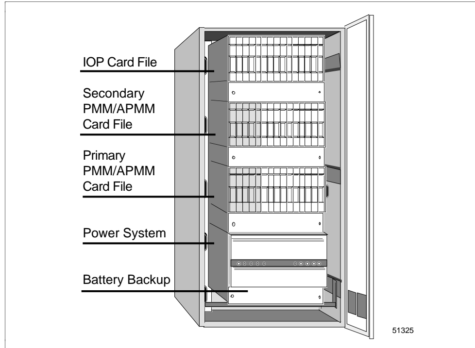
Figure 2-24 Single Cabinet with Redundant PMMs or APMMs
