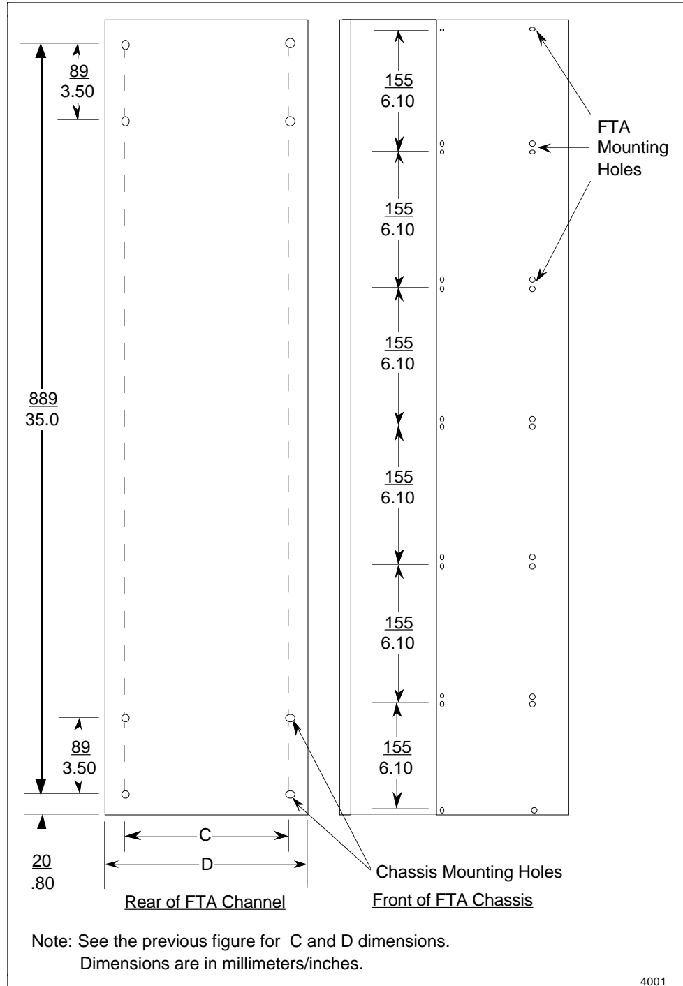
Figure 8-12 Vertical FTA Mounting Channel Installation Holes
