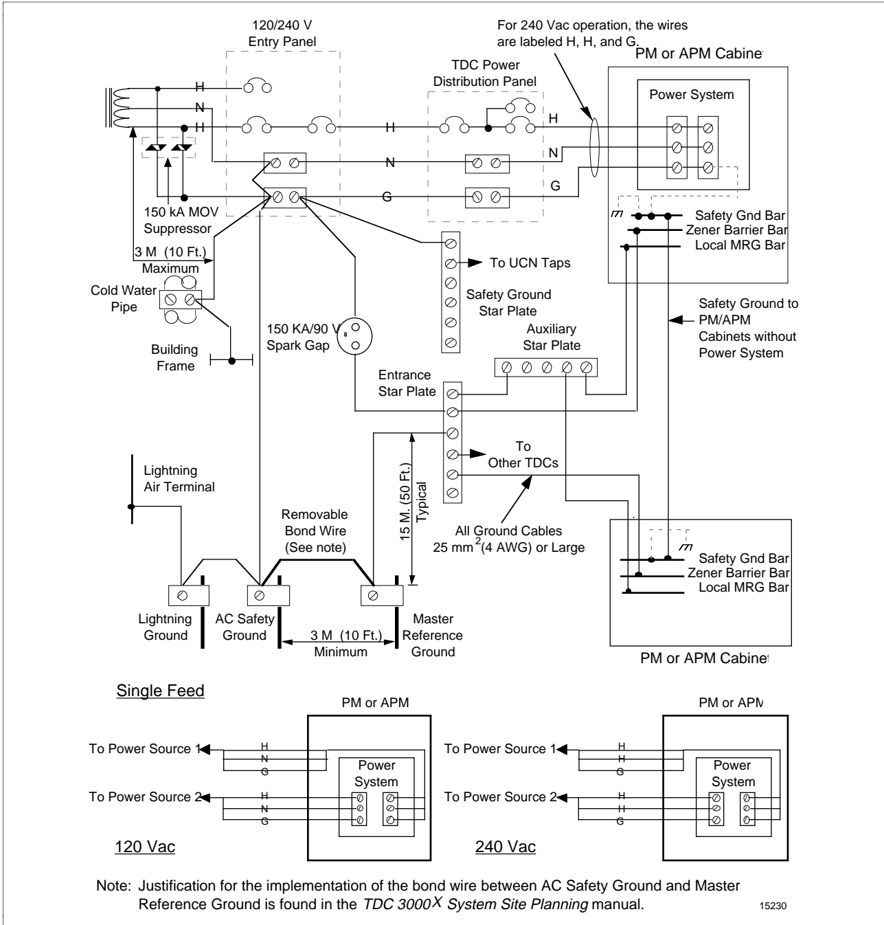
Figure 3-1 Subsystem AC Power and Ground Connections—Multiground System
