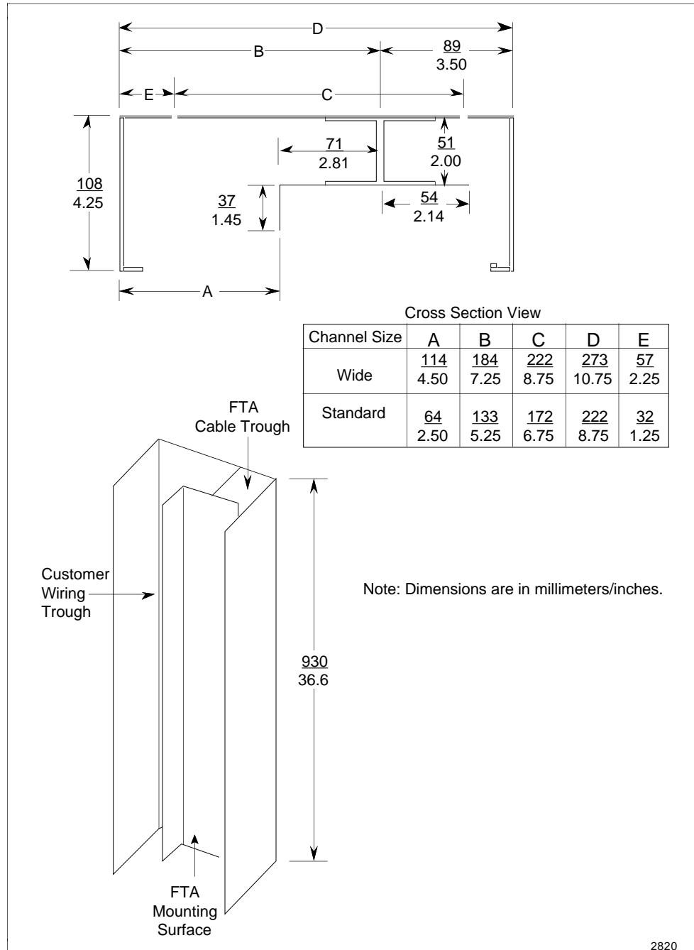
Figure 9-13 FTA Mounting Channel Dimensions
