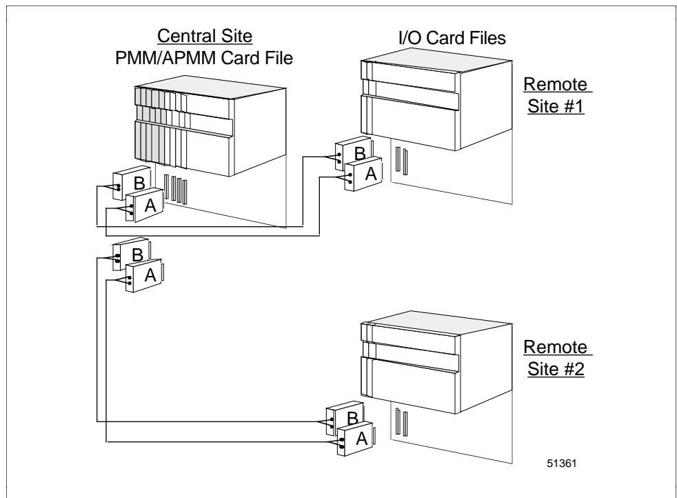
Figure 2-11 Long Distance I/O Link Extender Interconnections with Nonredundant PMM or APMM
