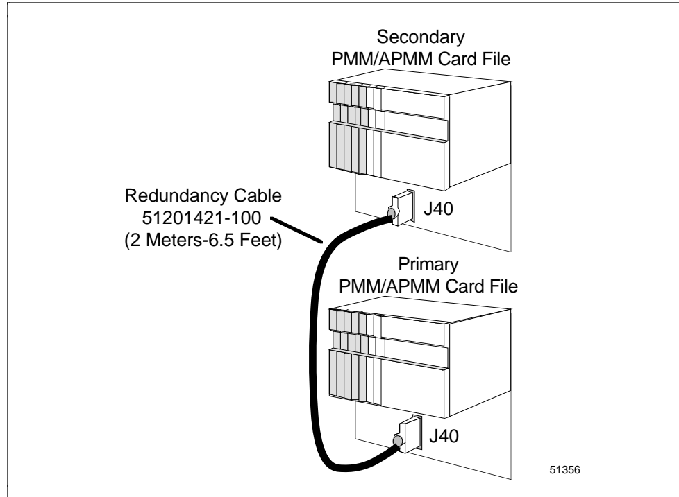
Figure 10-3 Redundant PMM or APMM Configuration Cabling
