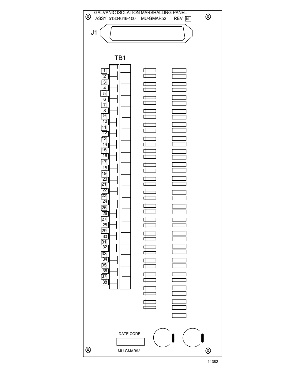
Figure 2-20 FTA Marshalling Panel Assembly Layout
