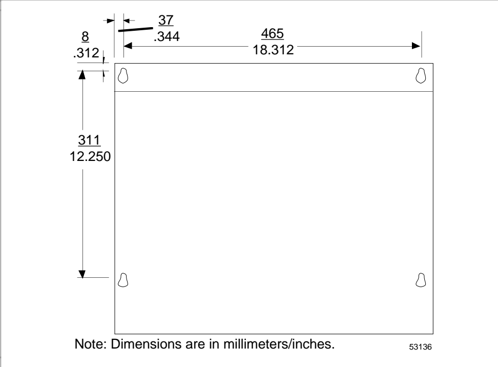
Figure 8-9 Power System Installation Dimensions
