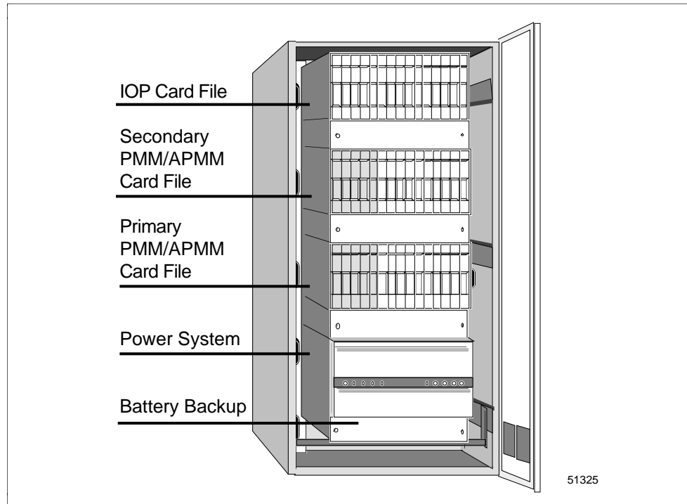
Figure 2-1 Redundant PMM or APMM Cabinet Layout
