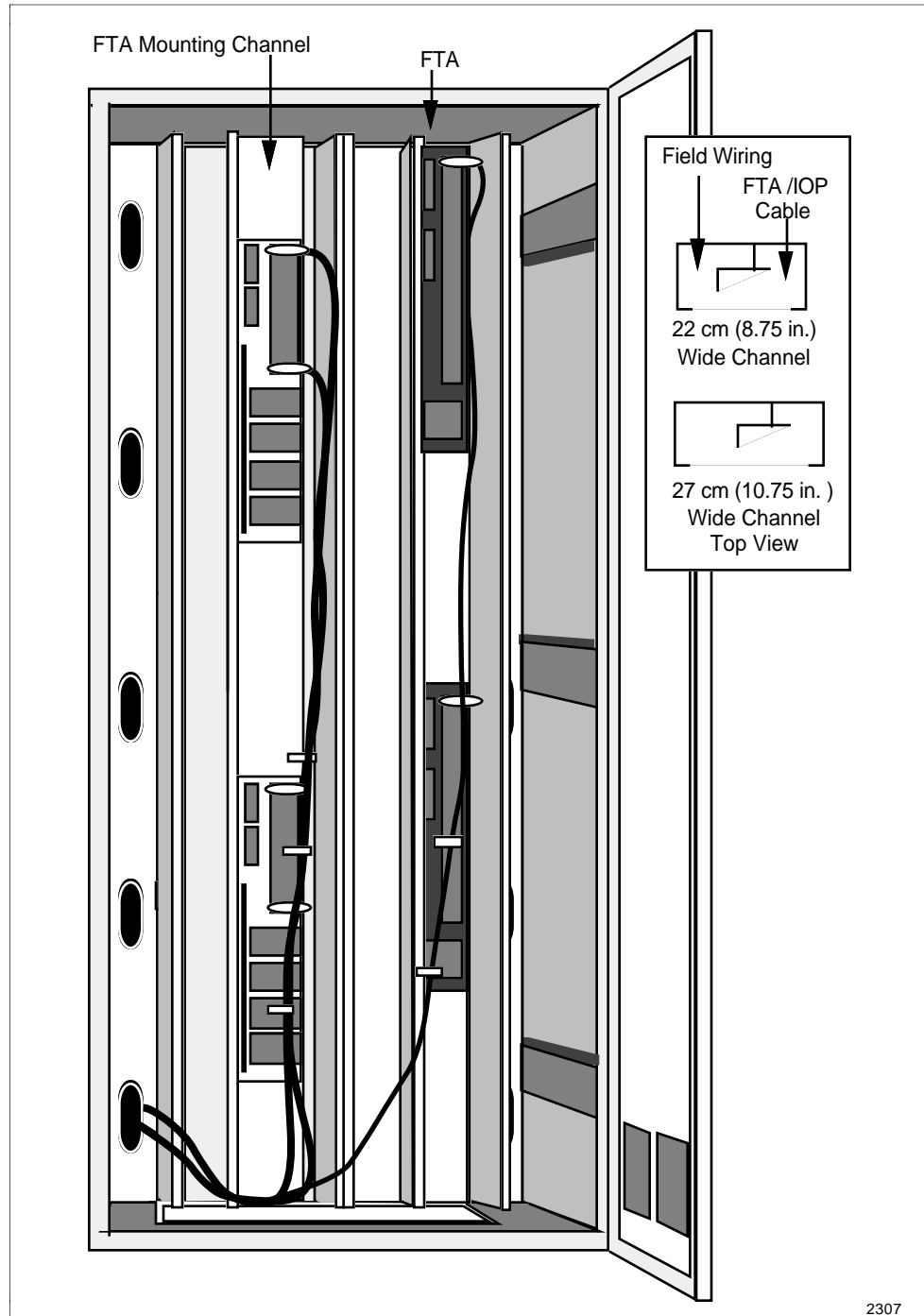
Figure 2-14 Typical Vertical FTA Mounting Channel Layout
