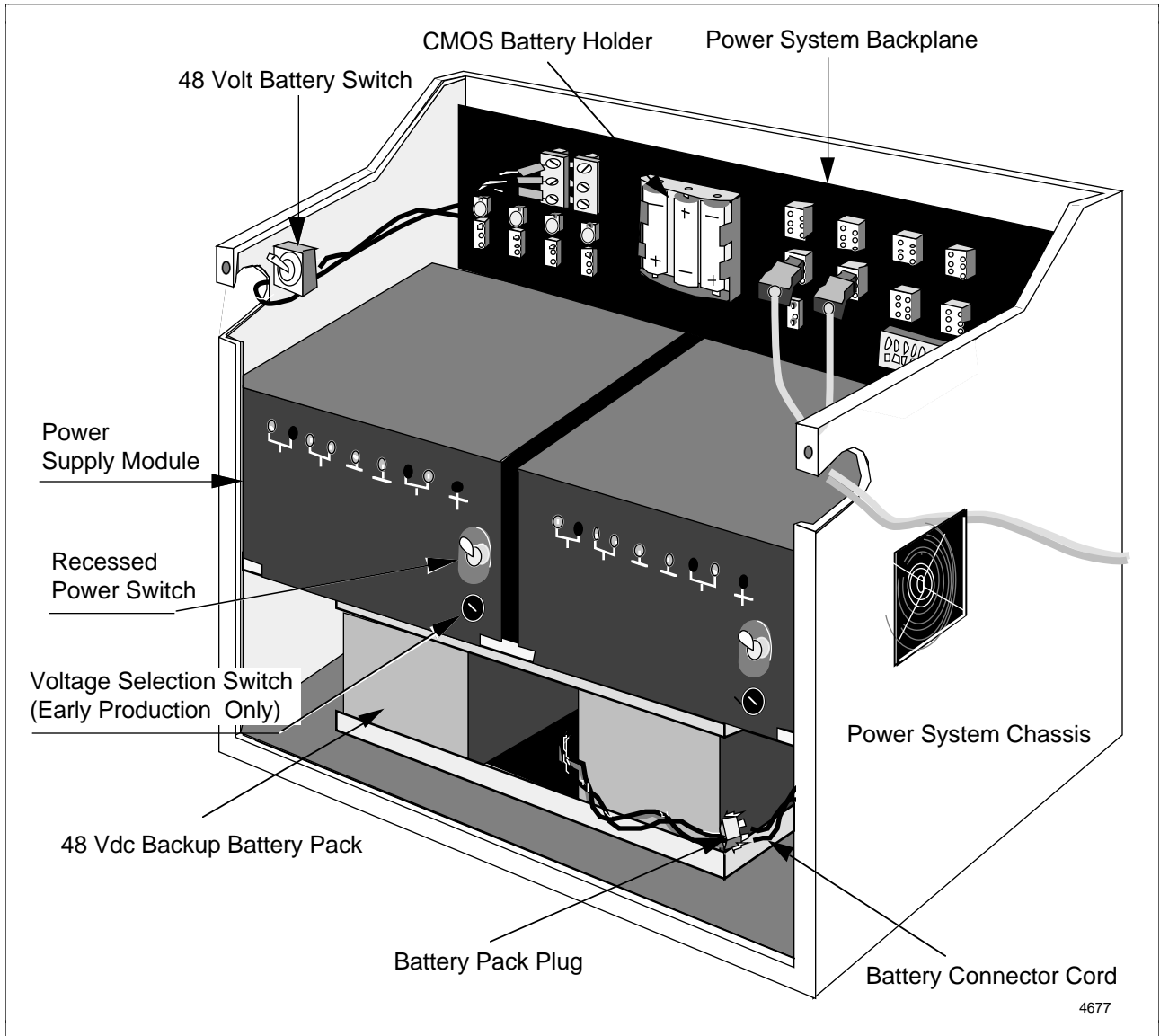
Figure 2-21 Standard Power System—Model MU-PSRX03
