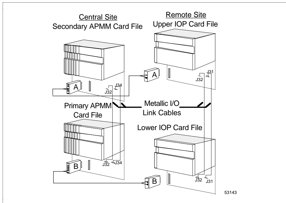
Figure 11-5 Remote Site Multi-IOP Card File I/O Link Interface Cabling
