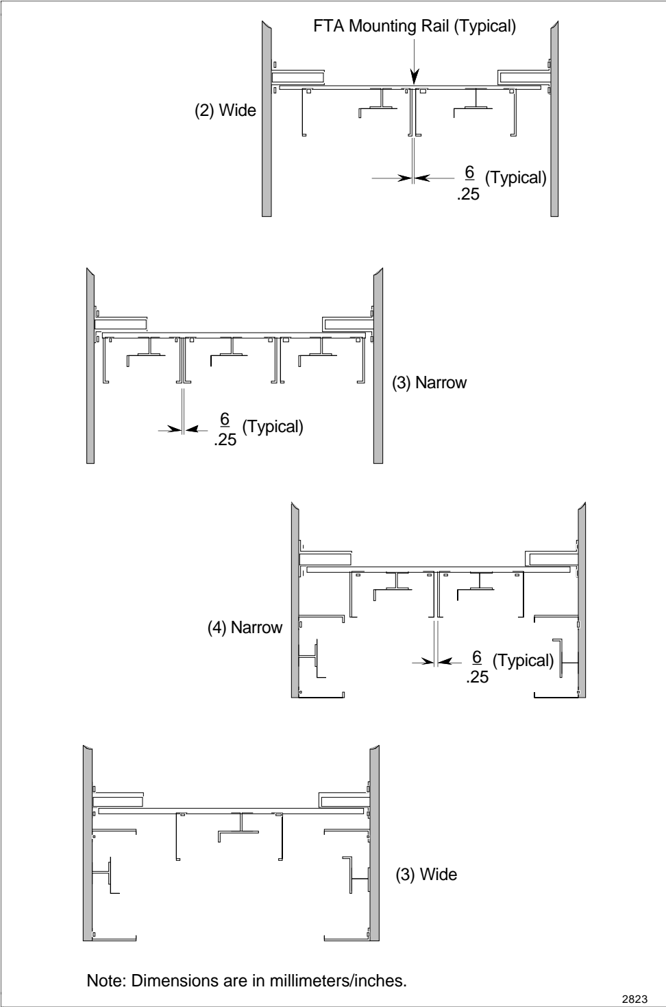
Figure 9-12 FTA Mounting Channel Configurations
