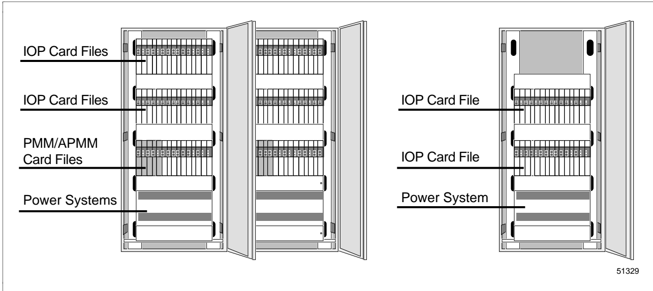
Figure 2-26 Dual Cabinet with Redundant PMMs or APMMs with Remote I/O Cabinet
