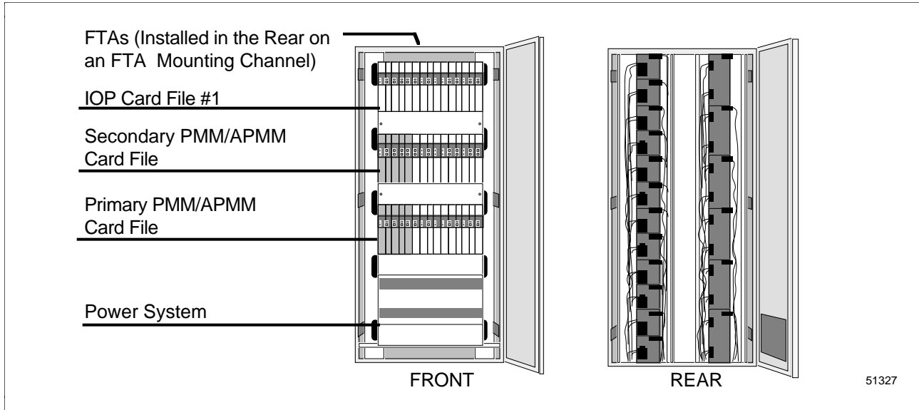
Figure 8-7 Typical Dual-Access Cabinet Assembly Layout
