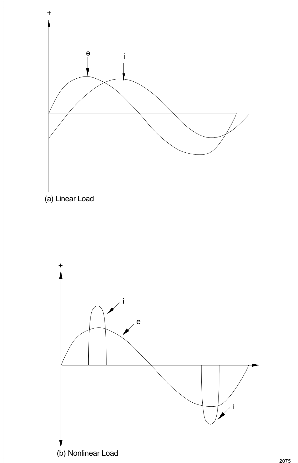
Figure 3-3 Crest Factor
