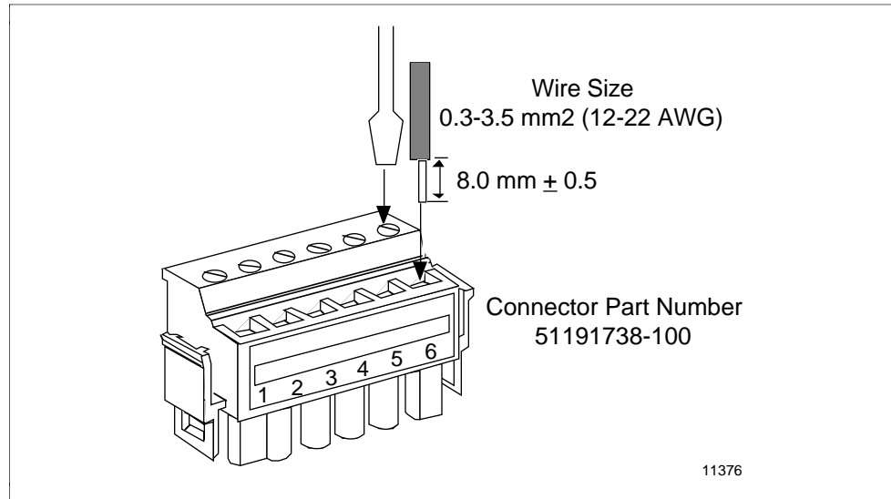
Figure 2-19 Compression-Type Galvanic Isolation Module Terminal Connector
