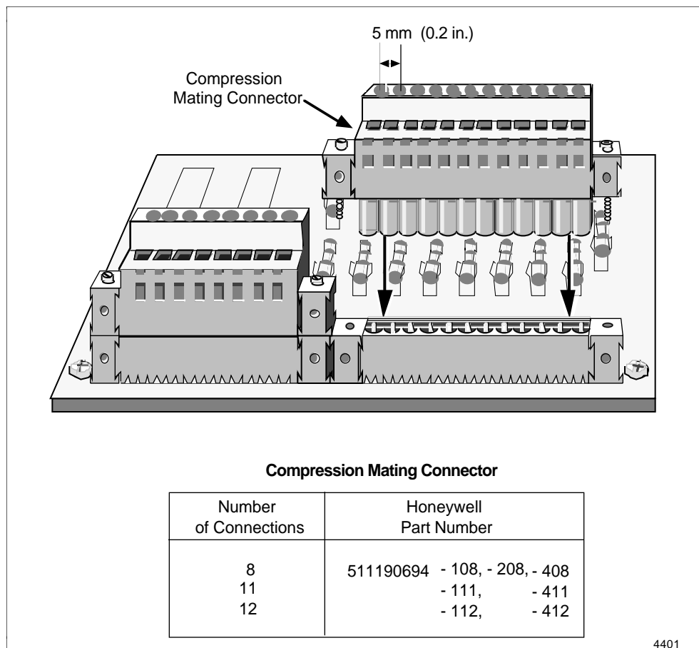
Figure 2-15 Typical FTA Compression Terminal Connector
