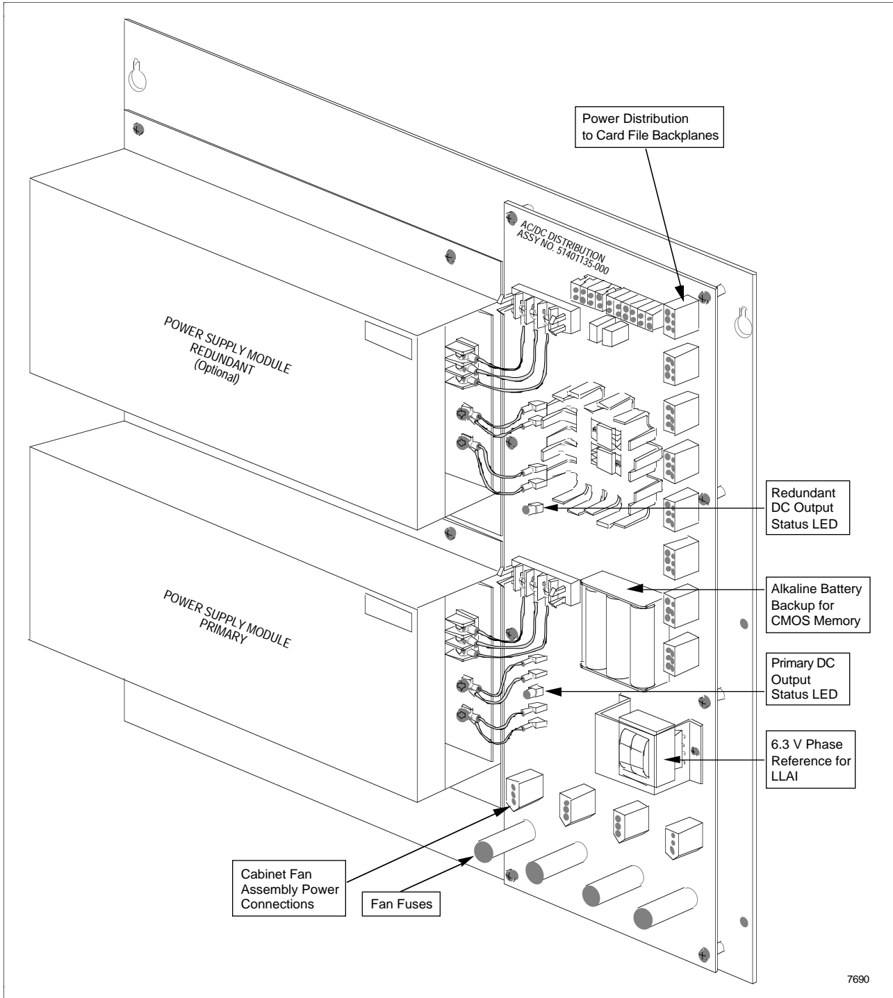
Figure 2-23 AC Only Power System—Not for CE Compliant Applications
