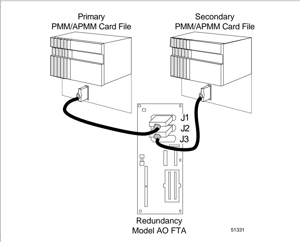
Figure 2-8 Analog Output FTA with Redundant Analog Output IOPs
