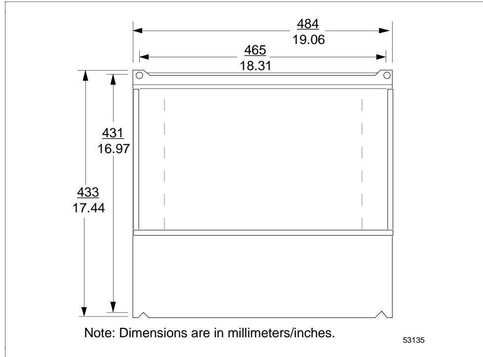
Figure 8-8 Card File Installation Dimensions
