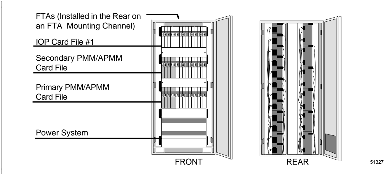
Figure 9-9 Typical Dual-Access Cabinet Assembly Layout
