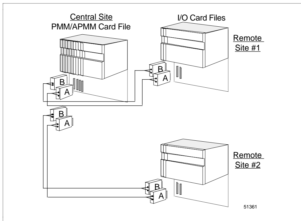
Figure 11-3 Long Distance I/O Link Extender Interconnections with Nonredundant PMM or APMM
