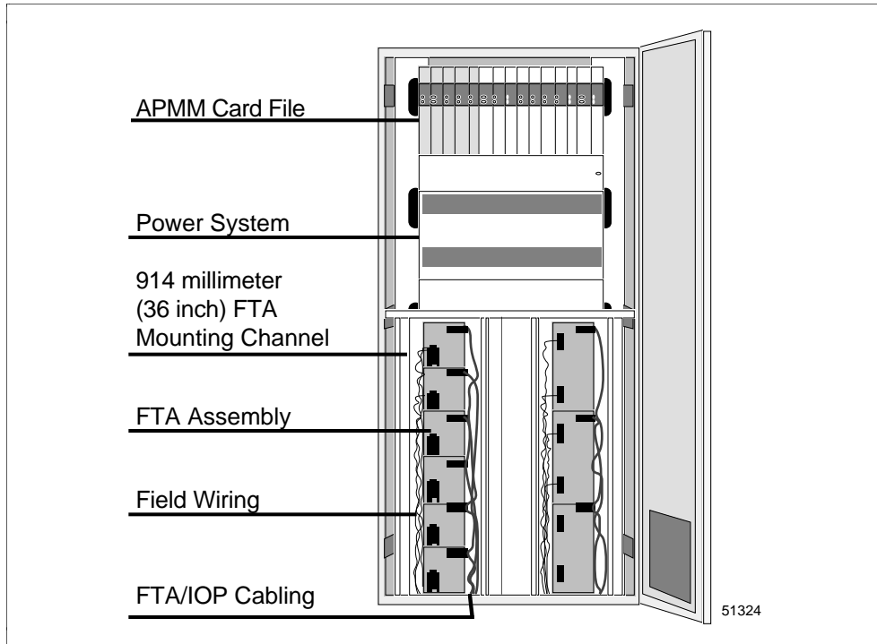
Figure 9-8 Typical Single-Access Cabinet Assembly Layout
