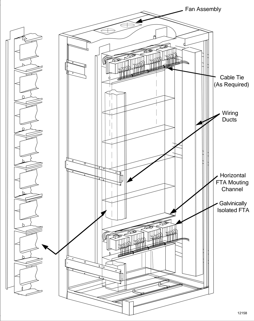
Figure 9-15 Horizontal FTA Mounting Channel Cabinet Layout
