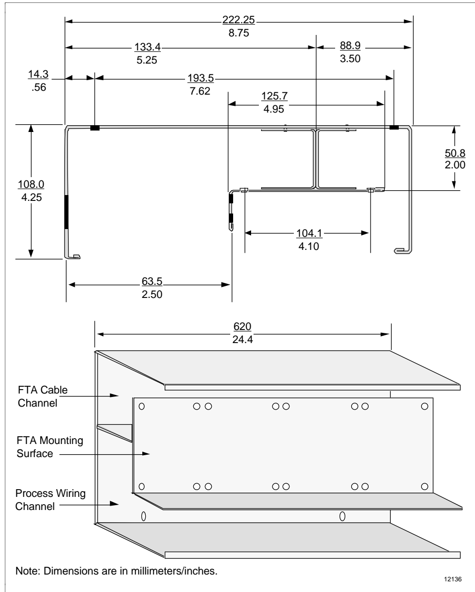
Figure 9-16 Horizontal FTA Mounting Channel Dimensions
