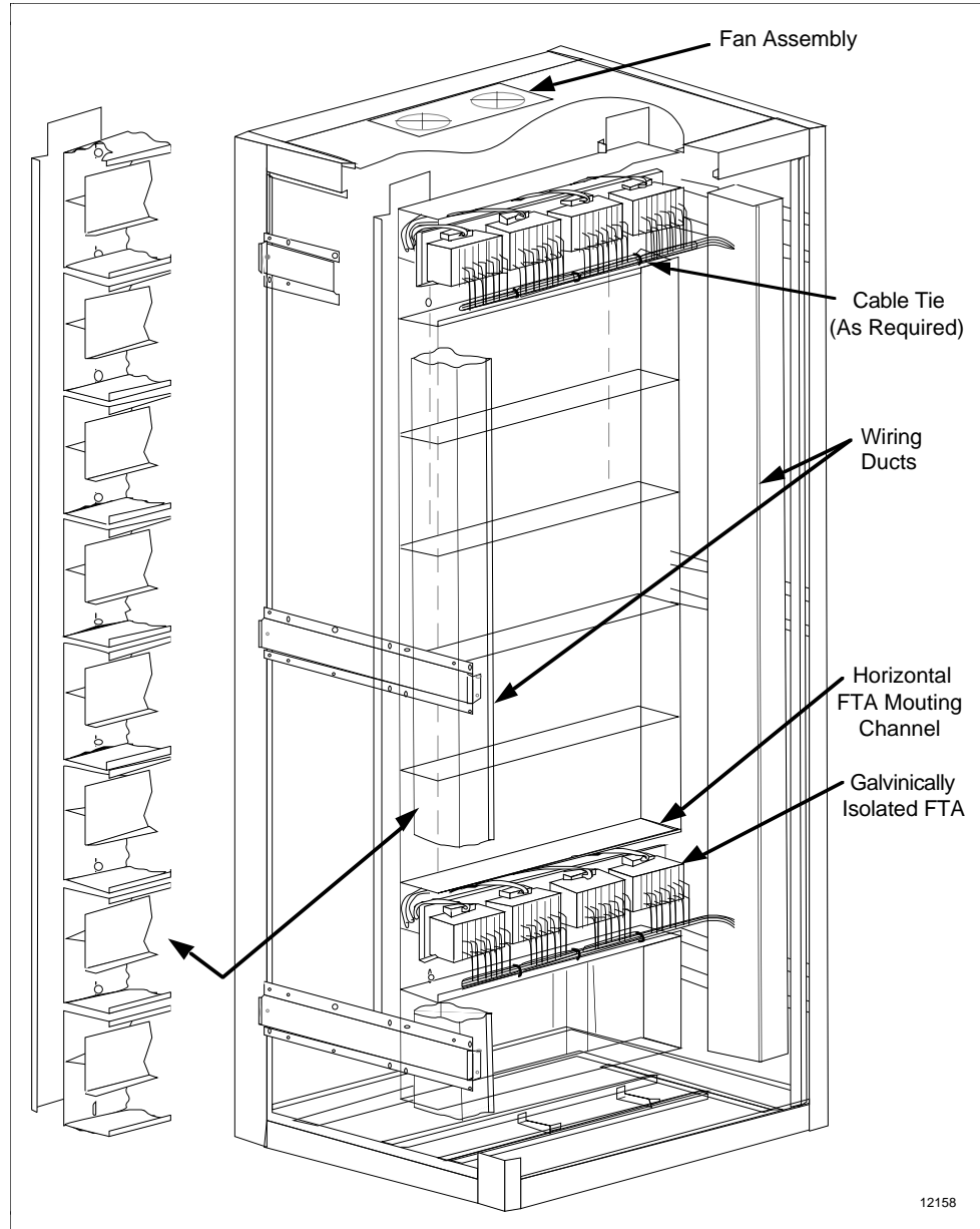
Figure 8-13 Horizontal FTA Mounting Channel Cabinet Layout
