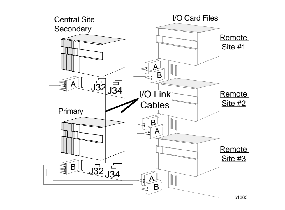
Figure 11-2 Standard I/O Link Extender Interconnections with Redundant PMMs or APMMs
