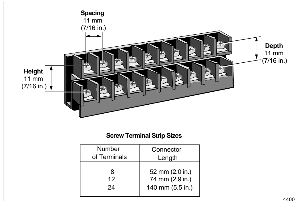
Figure 2-16 Typical FTA Fixed-Screw Terminal Connector
