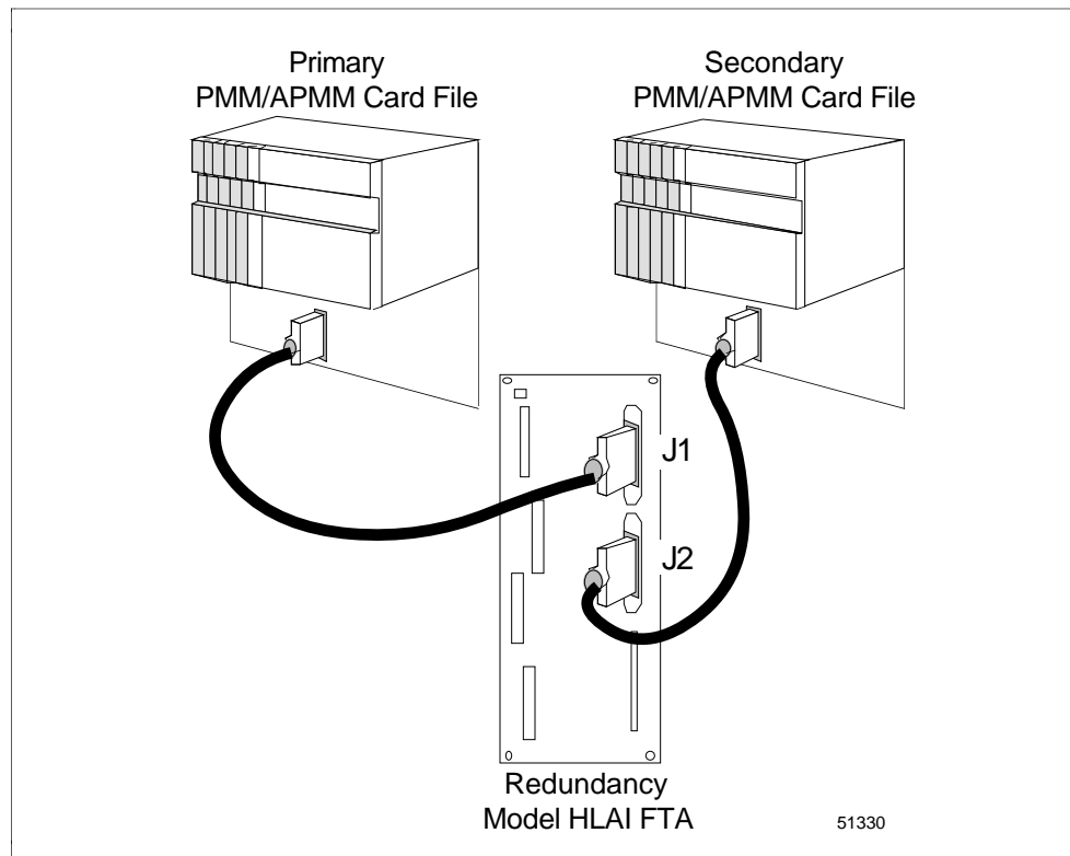
Figure 2-7 HLAI FTA with Redundant HLAI IOPs
