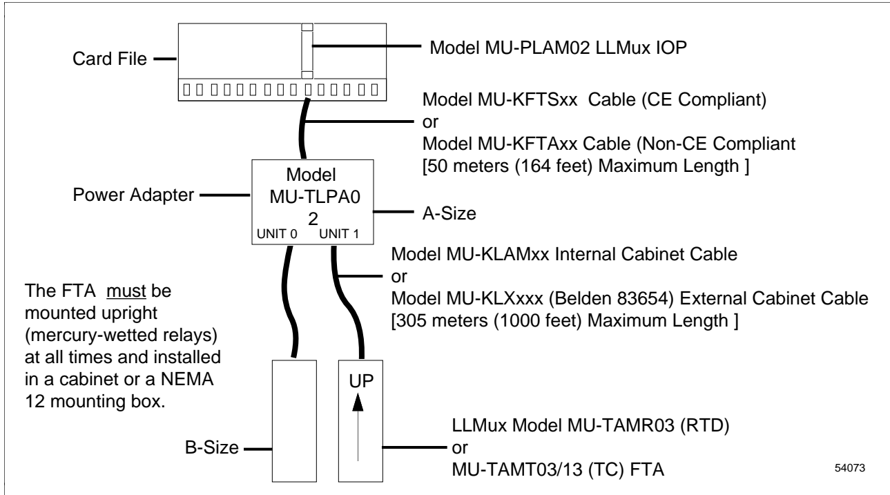
Figure 12-1 LLMux Configuration Interconnections—CE Compliant
