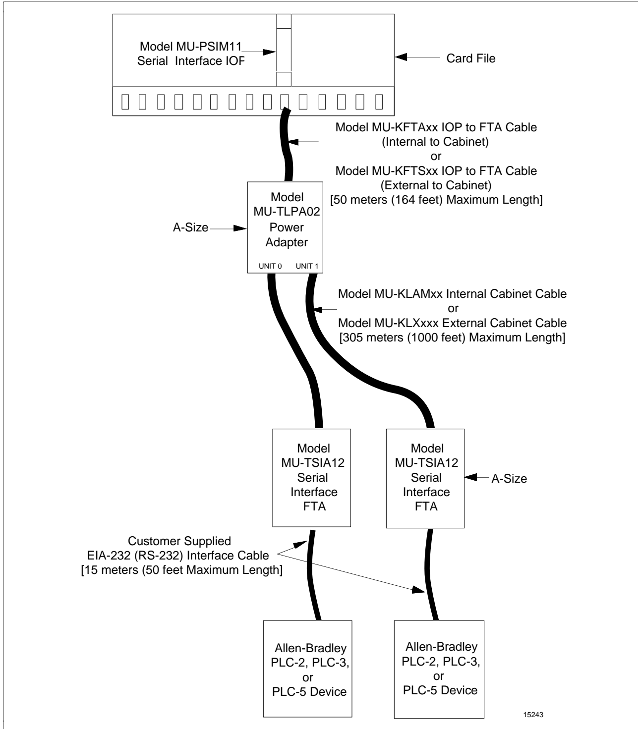
Figure 14-4 Model MU-TSIA12 Serial Interface FTA Interconnections—CE Compliant
