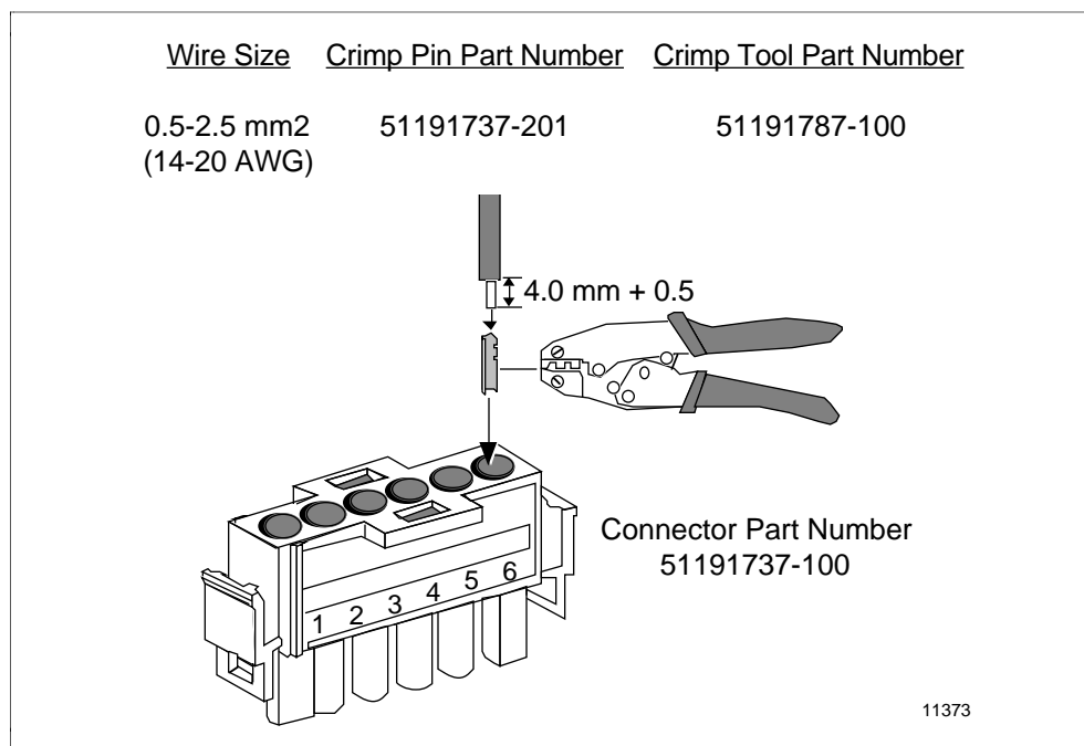
Figure 2-18 Crimp Pin-Type Galvanic Isolation Module Terminal Connector
