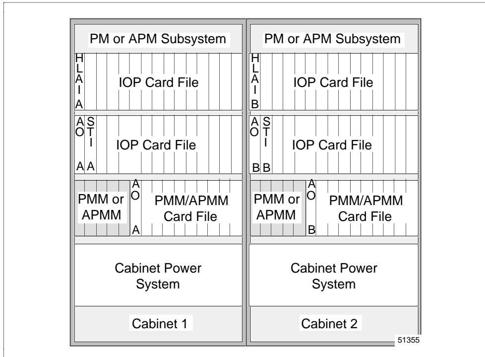
Figure 10-2 Dual Cabinet with Redundant PMMs or APMMs
