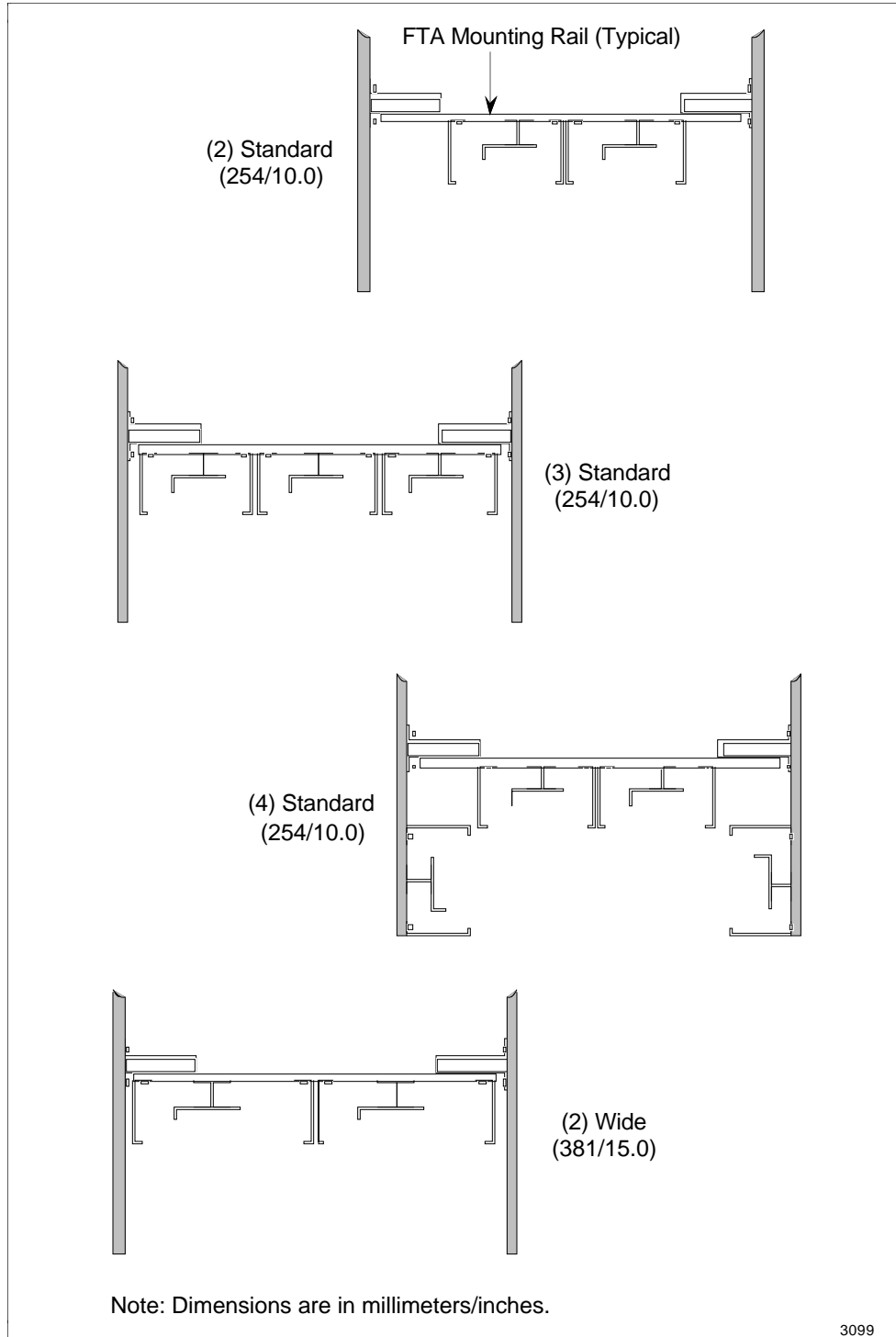
Figure 8-10 Typical Vertical FTA Mounting Channel Configurations
