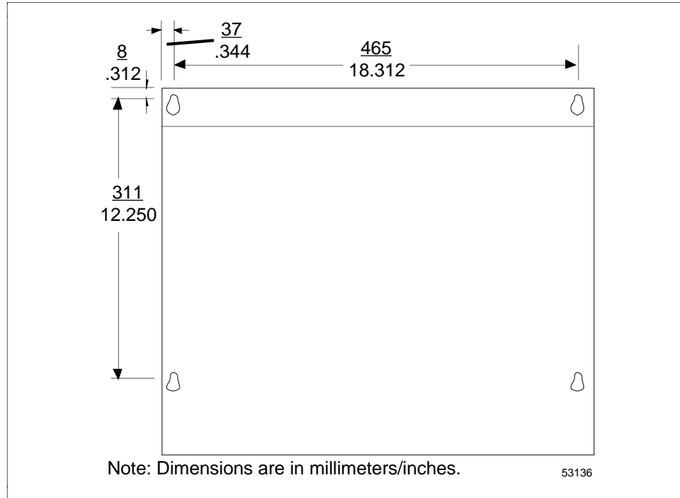
Figure 9-11 Power System Installation Dimensions
