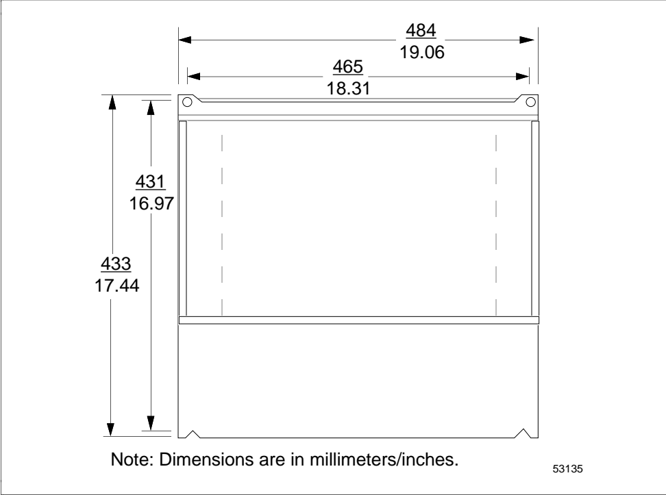
Figure 9-10 Card File Installation Dimensions
