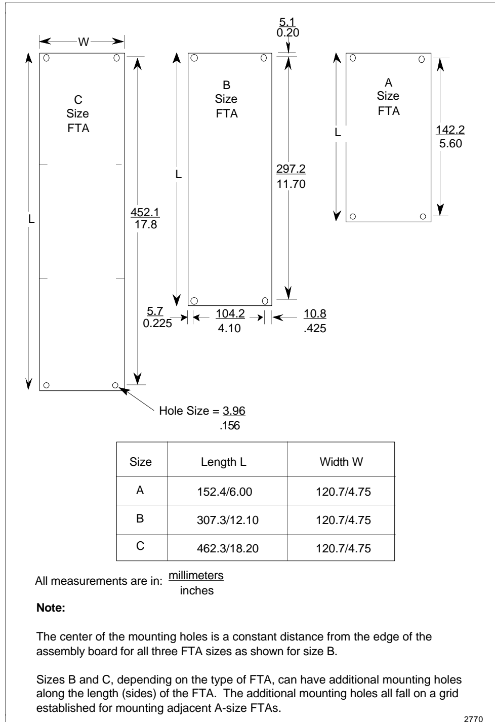
Figure 2-13 Field Termination Assembly (FTA) Sizes
