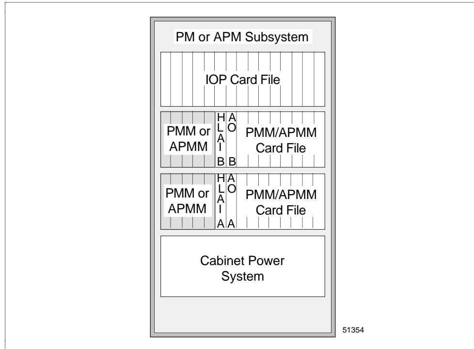
Figure 10-1 Single Cabinet with Redundant PMMs or APMMs
