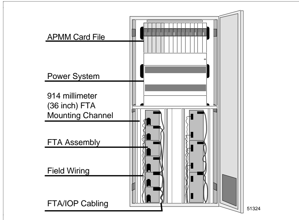
Figure 8-6 Typical Single-Access Cabinet Assembly Layout
