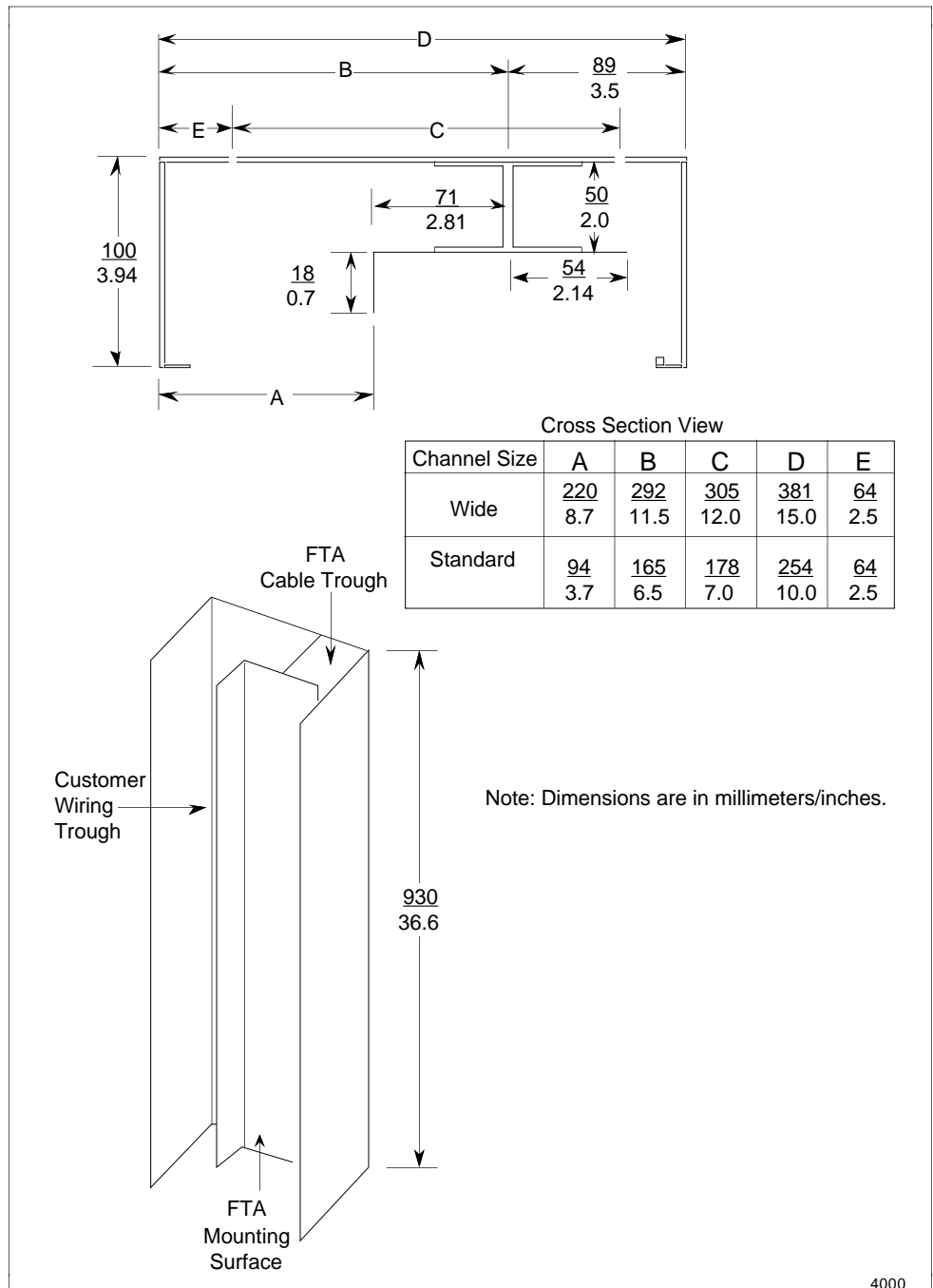
Figure 8-11 Vertical FTA Mounting Channel Dimensions
