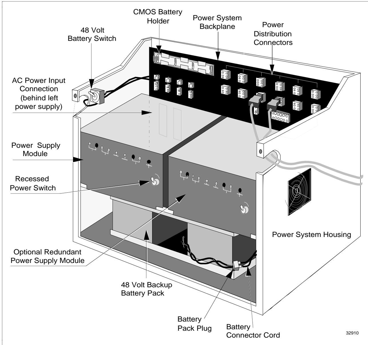
Figure 2-22 Standard Power System—Model MU-PSRX04
