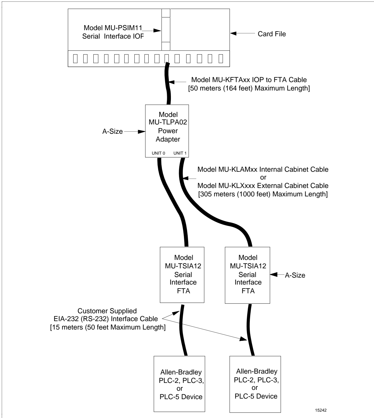
Figure 14-3 Model MU-TSIA12 Serial Interface FTA Interconnections—Non-CE Compliant
