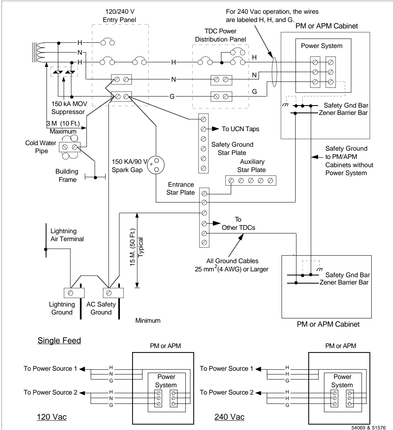
Figure 3-2 Subsystem AC Power and Ground Connections— Single-Ground System
