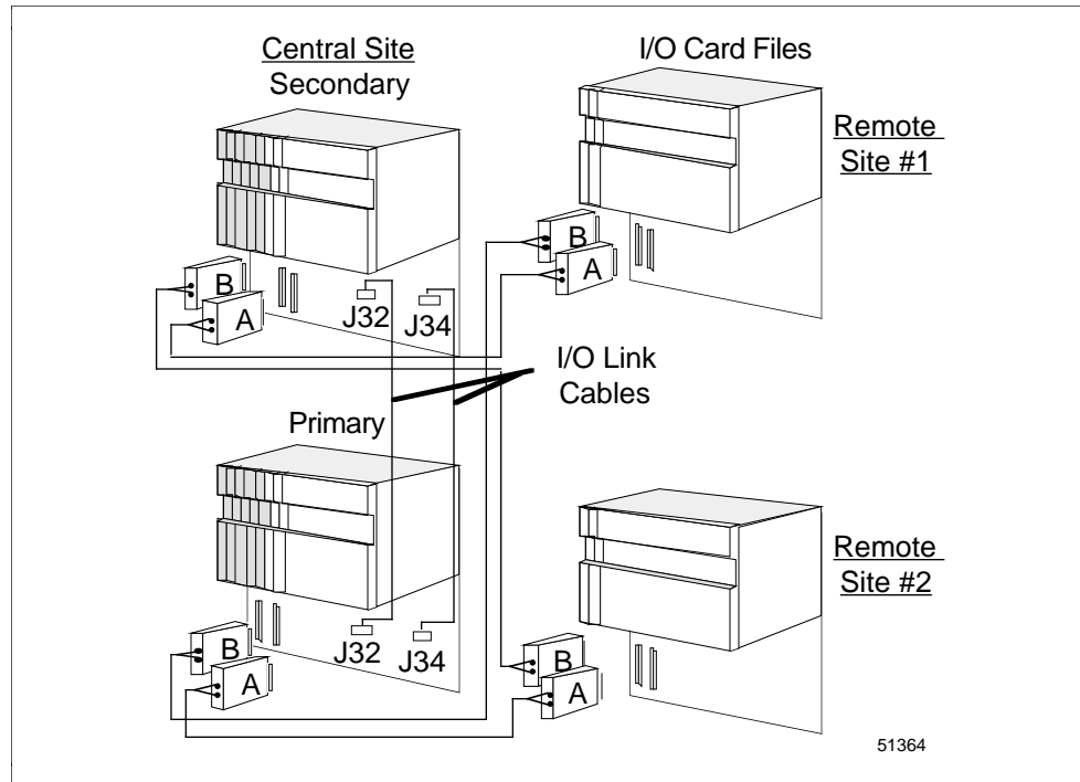
Figure 11-4 Long Distance I/O Link Extender Interconnections with Redundant PMMs or APMMs
