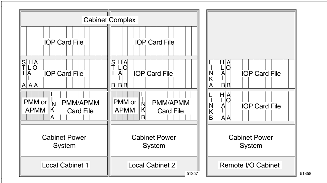
Figure 10-4 Local/Remote Cabinet Configuration
