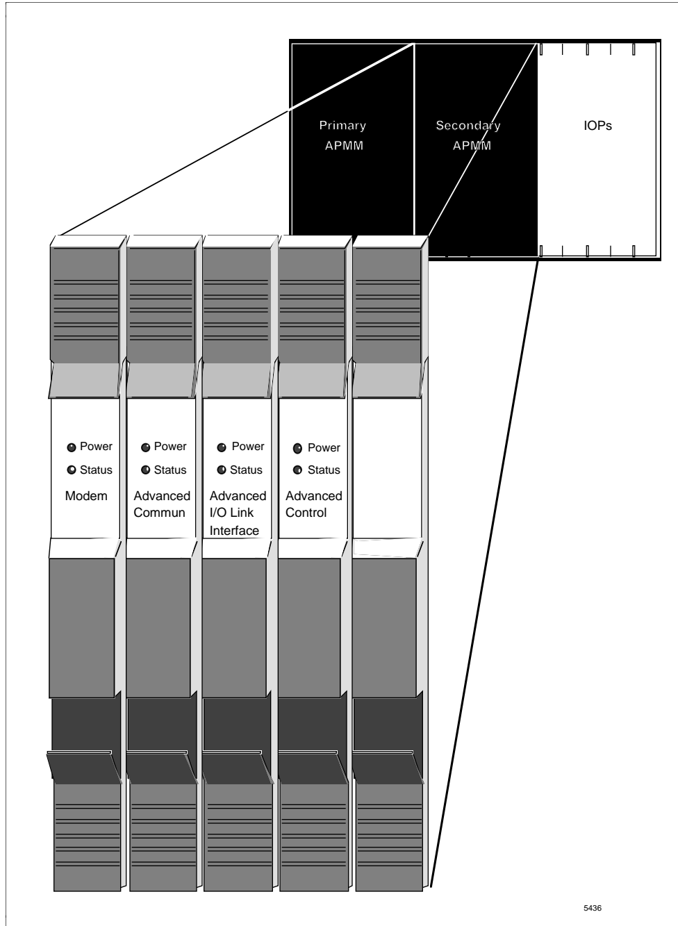
Figure 2-5 Redundant APMM Card File
