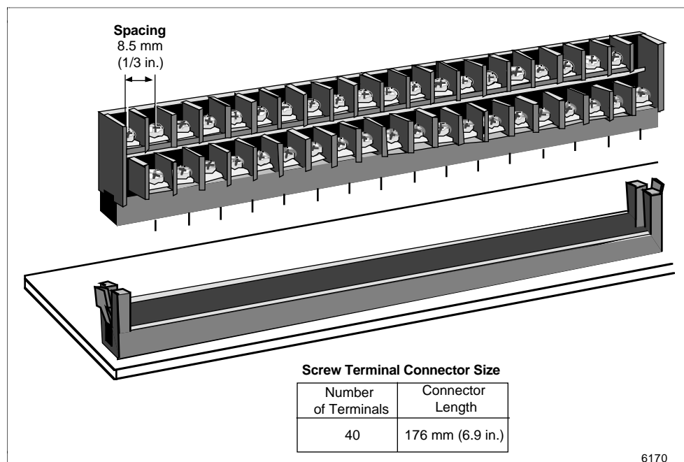
Figure 2-17 Typical FTA Removable-Screw Terminal Connector
