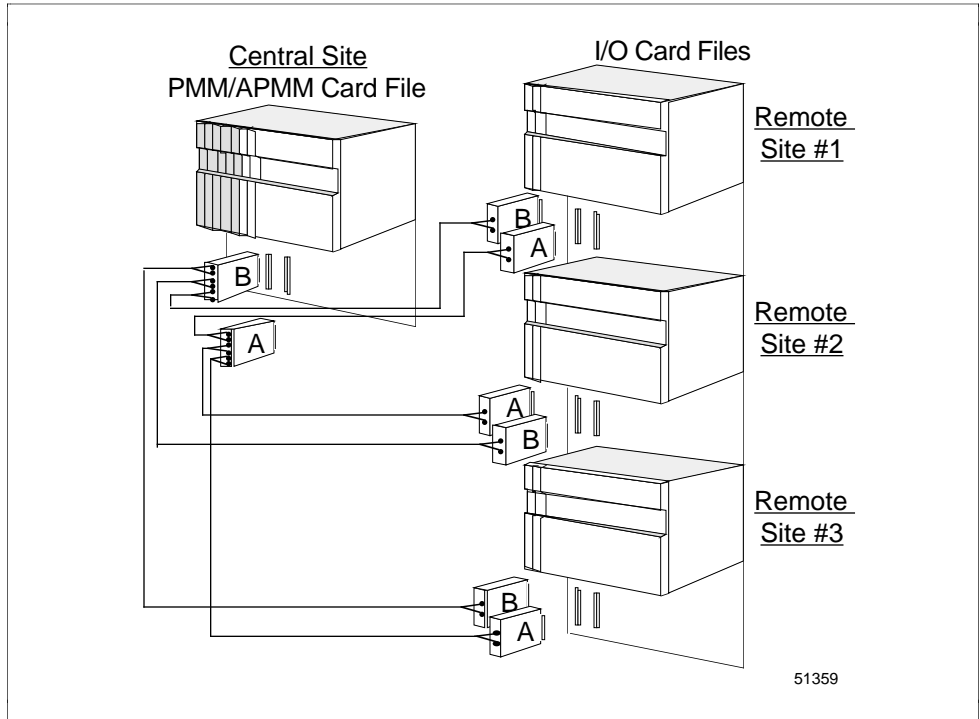
Figure 2-9 Standard I/O Link Extender Interconnections with Nonredundant PMM or APMM
