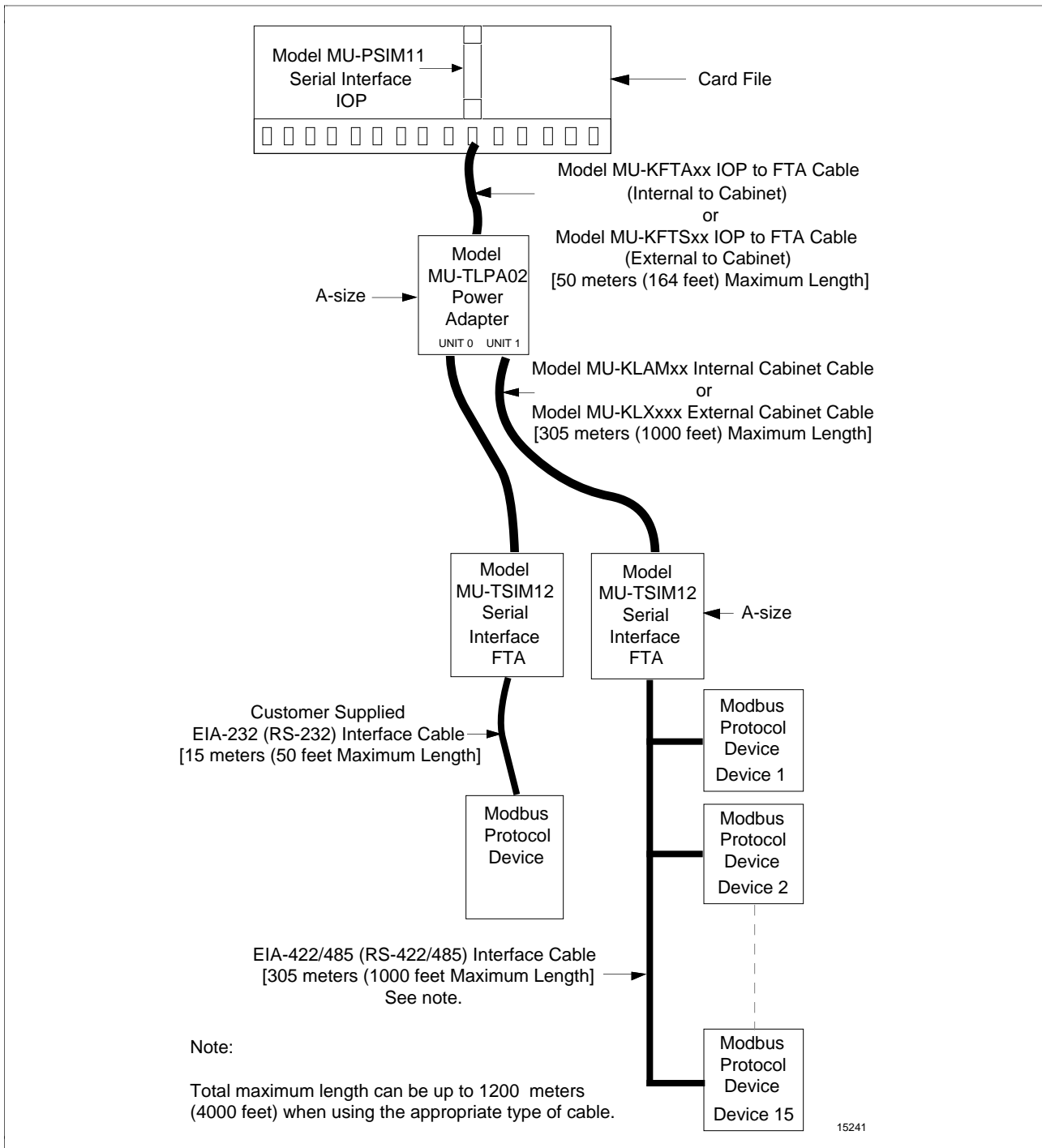
Figure 14-2 Model MU-TSIM12 Serial Interface FTA Interconnections—CE Compliant
