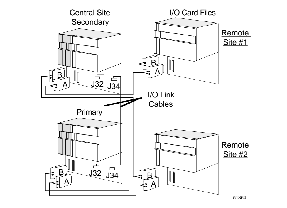
Figure 2-12 Long Distance I/O Link Extender Interconnections with Redundant PMMs or APMMs
