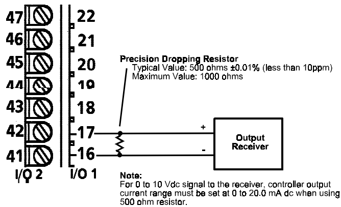
Figure 3-8. Built-in Milliampere Output Connections
