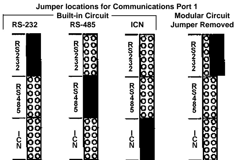
Figure 5-2. Locations for Port 1 Communications Jumper
