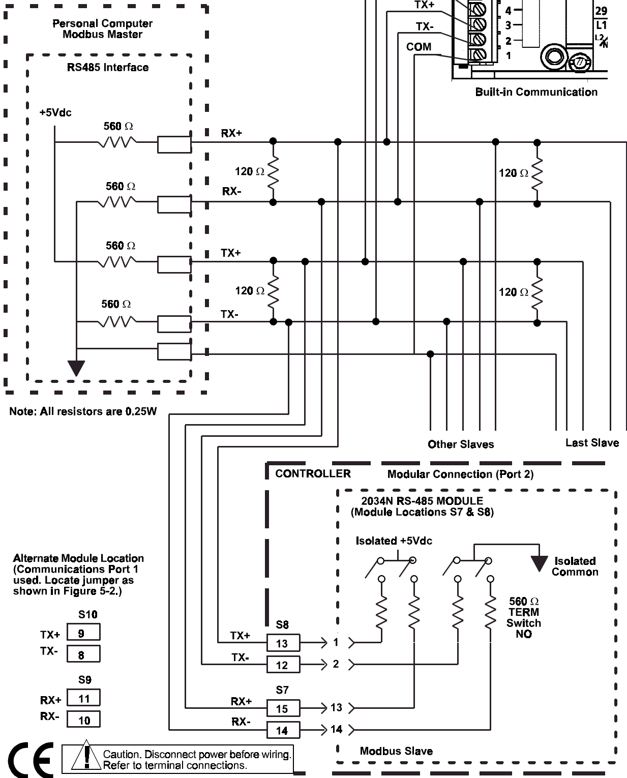
Figure 5-8. Typical Modbus Connections for an RS-485, 4-Wire Network (Slave Controller)
