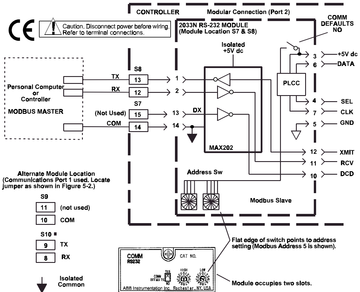
Figure 5-5. Typical Network Connections for Modular Modbus RS-232 Communication
