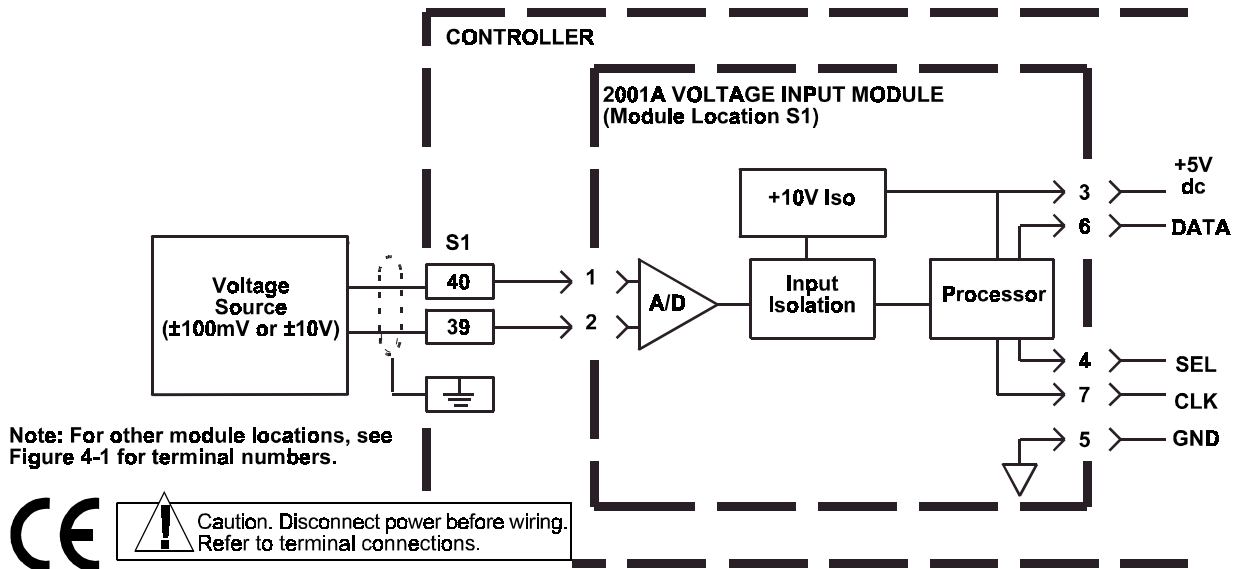
Figure 4-7, Typical Connections for a 2001A Voltage Input Module
