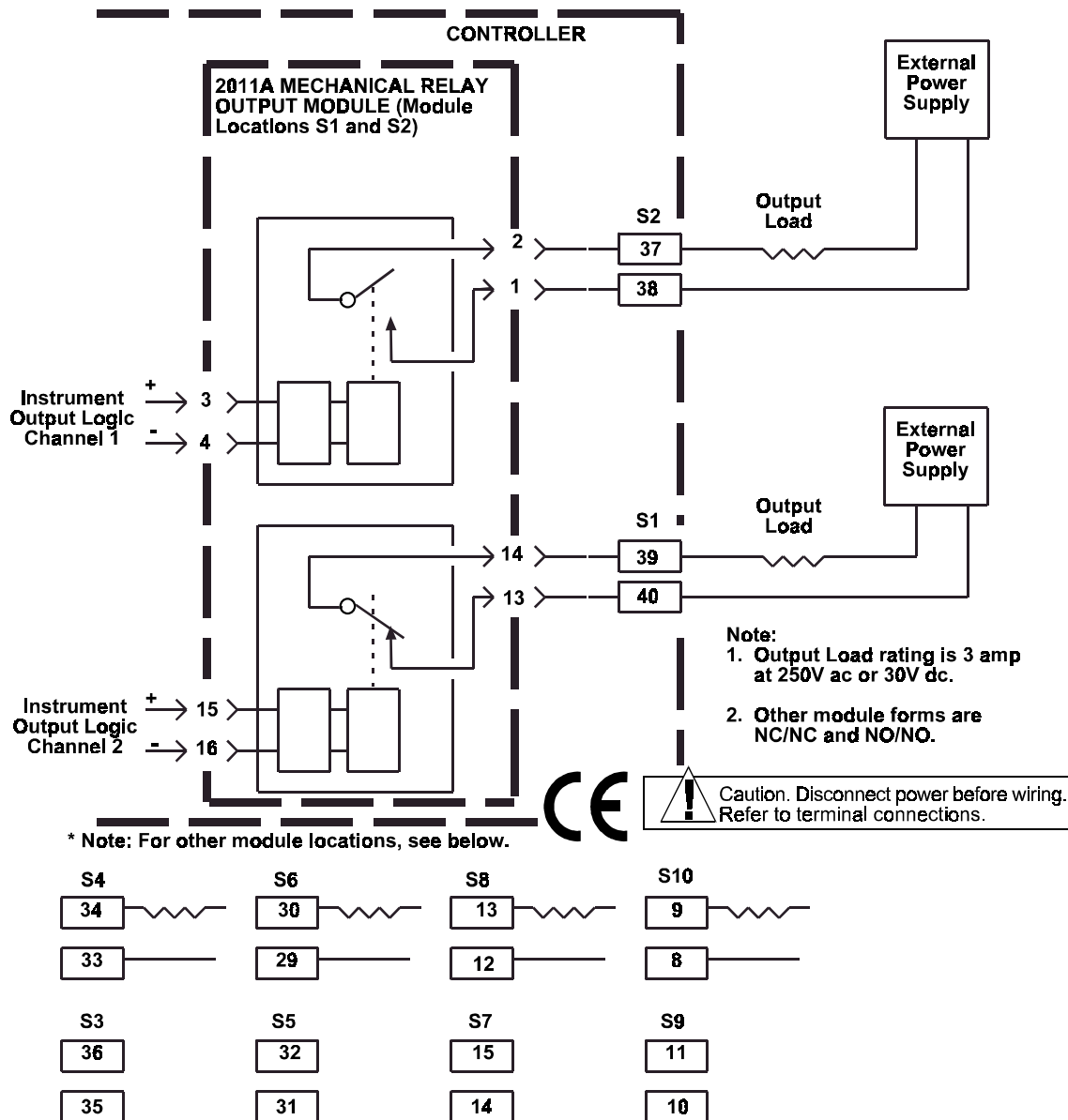
Figure 4-14. Typical Connections for a 2011A Mechanical Relay Output Module (Dual SPST, NO/NC)
