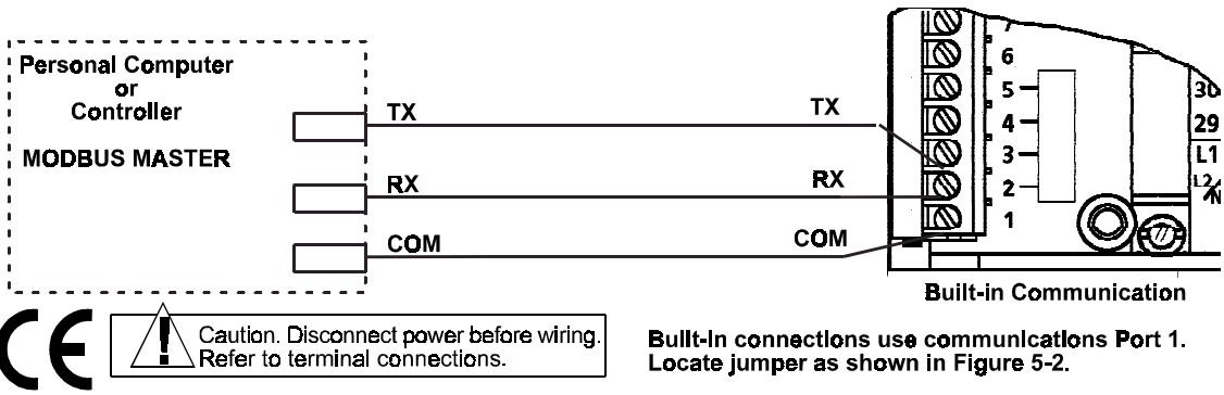
Figure 5-4. Typical Network Connections for Built-In Modbus RS-232 Communication
