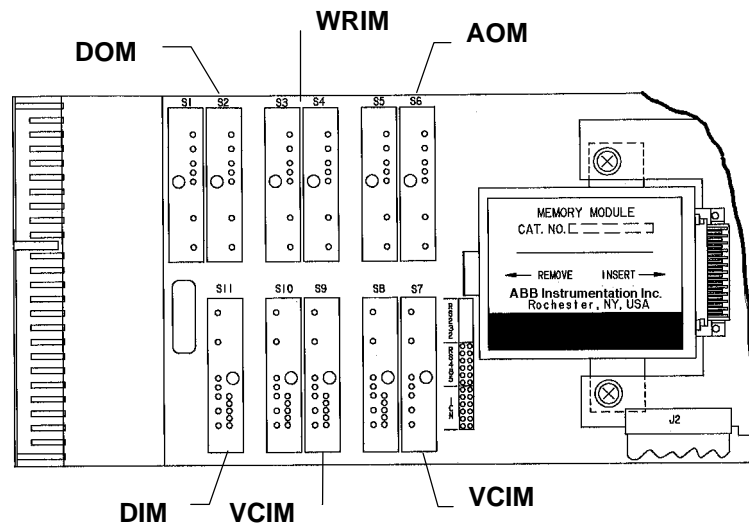
Figure 2-1. Example of an I/O Planning Form for a Controller with I/O Modules
