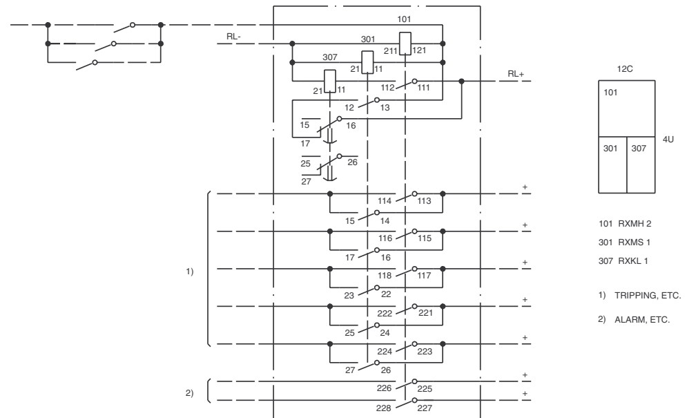
Fig. 5 High-speed tripping assembly, RK 651 231-AB, Diagram No. 5651 109-AB
