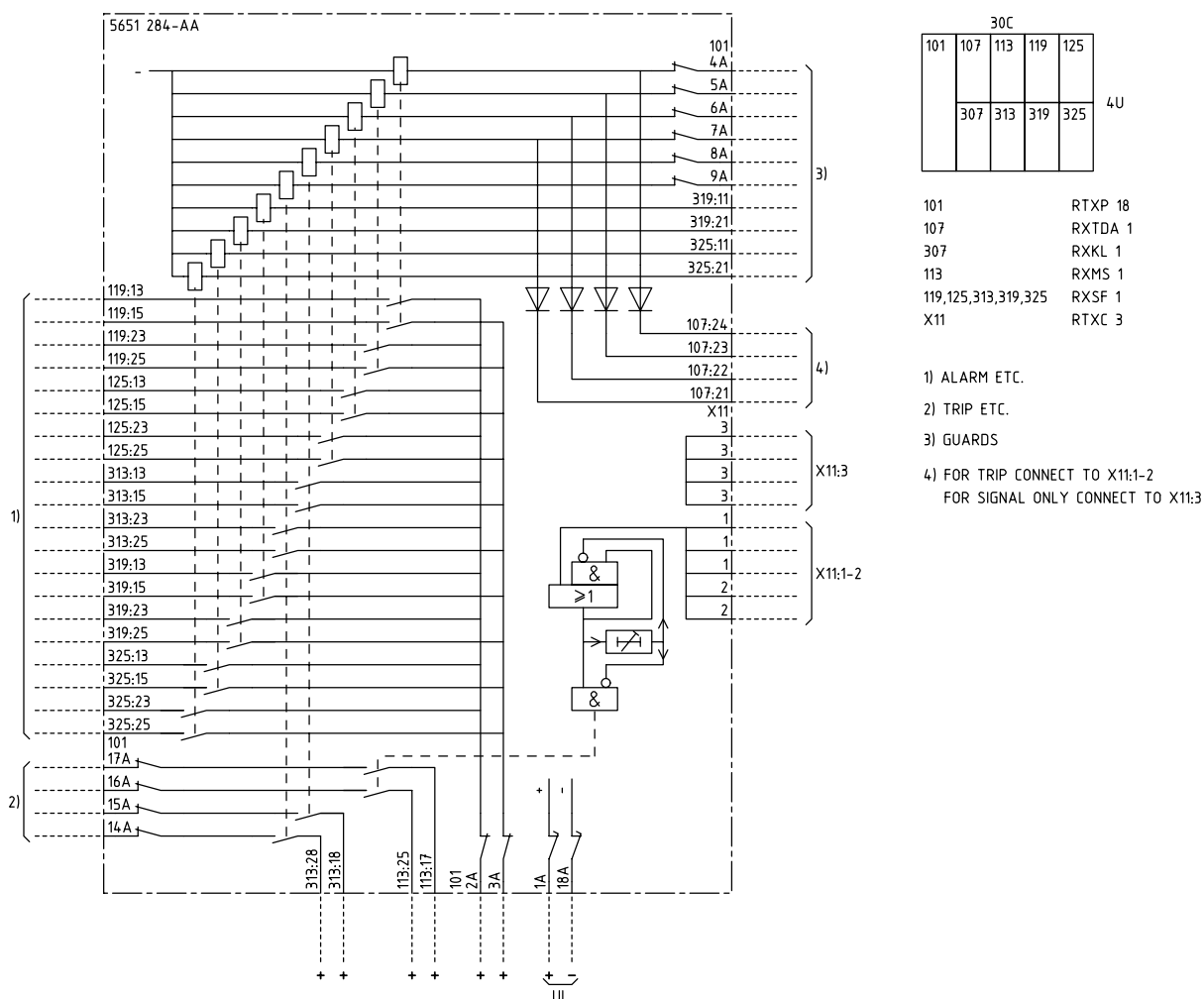
Fig. 6 Auxiliary trip unit, RK 891 031-AA, Diagram No. 5651 284-AAA
